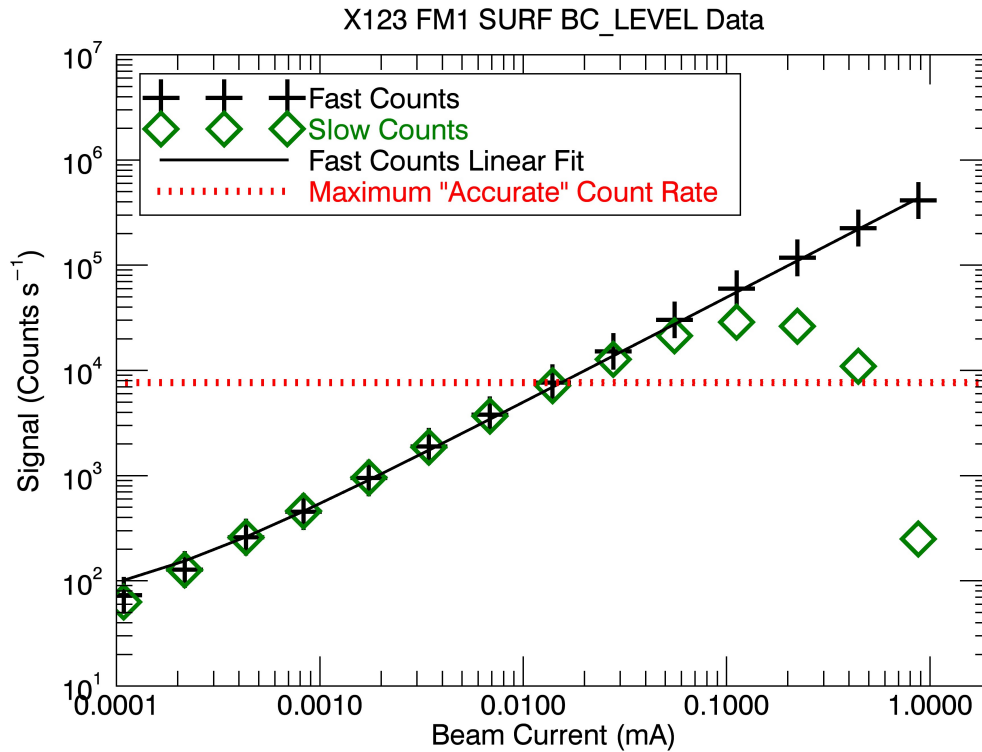
Figure 8.15: NIST SURF X123 linearity test shows a maximum count rate limit of \sim 8,000 counts s^{-1} , for an accurate spectrum. Maximum count rate is deduced from the last measured count rate, the red dotted lines, where the X123 slow counter (peaking time = 4.8 s), the green diamonds, and fast counter (peaking time = 100 ns), the black pluses, begin to diverge. The black solid line is a linear fit to the fast counts. The SURF flux spectrum depends linearly with the SURF beam current ( I_e ), so a linear increase in the SURF beam current leads to a linear increase in the SURF photon flux.
