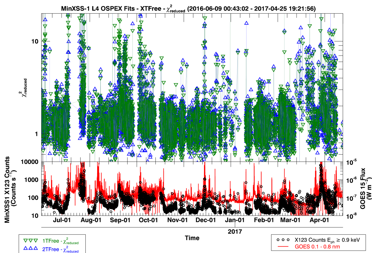
Figure 9.6: Reduced Chi-square ( \chi^2_{reduced} ) over the MinXSS-1 mission of 15 minute averaged X123 data fit by OSPEX 1TFree (green) and 2TFree (blue) class models. Values near unity are desired. The \chi^2_{reduced} is around 2 - 6 for most fits, which is OK. The MinXSS-1 X123 counts for E \geq 0.9 keV are plotted as the black circles in the bottom panel. The GOES 0.1 - 0.8 nm flux is plotted as the red line below to serve as a reference for the solar activity level.
