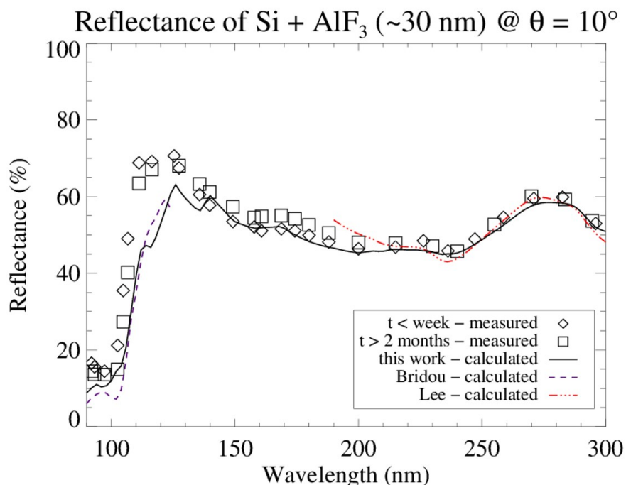
Figure 5.4: UV (90 – 300 nm) near-normal ( \theta = 10^\circ ) absolute reflectance measurements for \sim 30 nm of AlF 3 on Si for two samples, one deposited and measured within 1 week (diamonds) and the other measured after storage in the JPL MDL glove box for 2 months (squares). Performance differences are within measurement uncertainties ( \sim \pm 5\% ) indicating that the optical performance is not strongly modified by MDL glove box storage. Measurements follow the general spectral shape from calculated values of this work (black solid line), Bridou (blue dashed line; thermal evaporation) and Lee (red dash-dotted line; magnetron sputtered).
