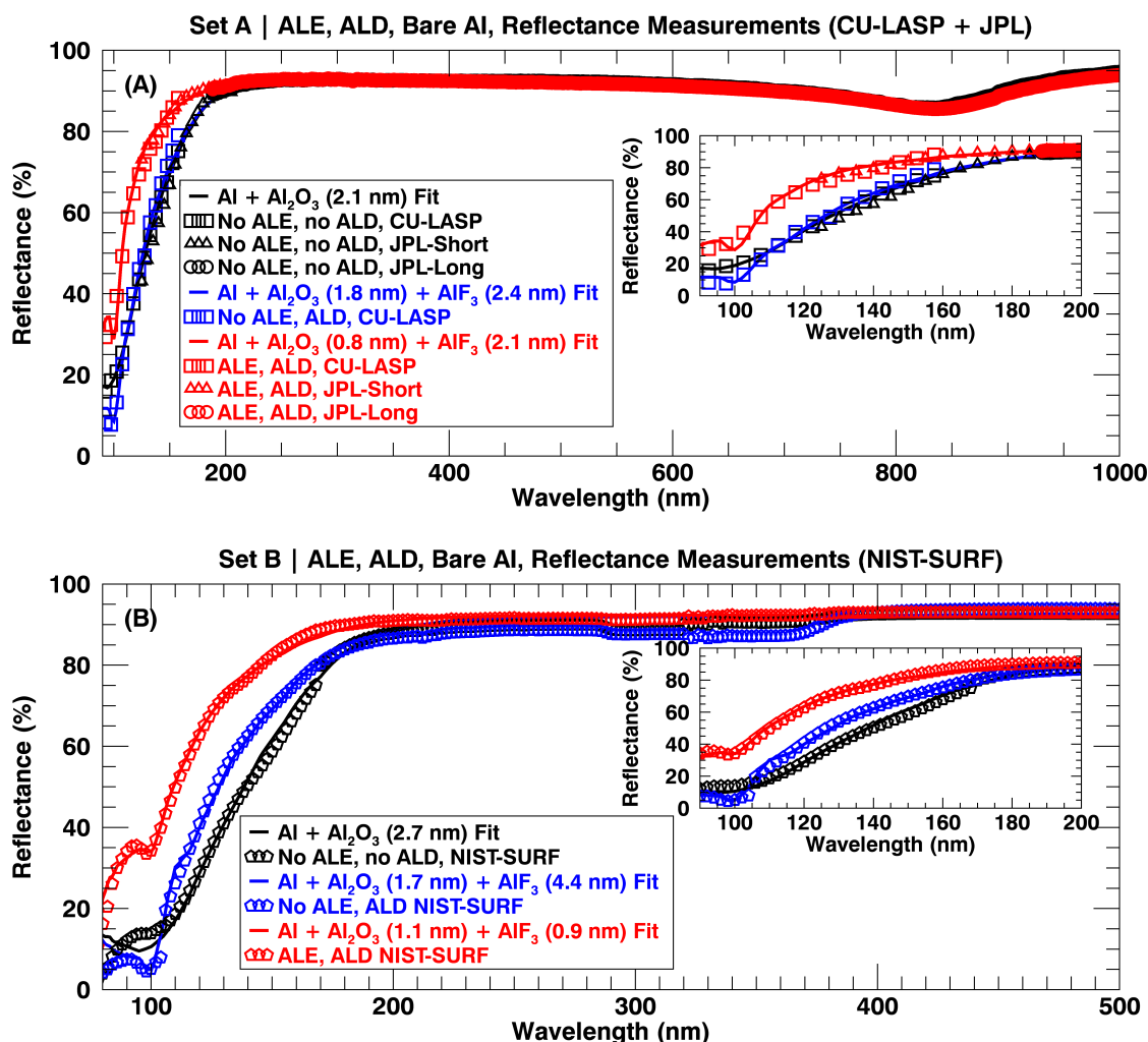
Figure 5.13: (A) Set A CU-LASP and JPL reflectance measurements (symbols) of Al-only (black), Al-ALD-AlF 3 (Blue) and Al-ALE-ALD-AlF 3 (red) show the etched sample achieves values near 30% at 90 nm while maintain high reflectance out to 250 nm. (B) Set B NIST-SURF reflectance measurements reaffirm the CU-LASP and JPL results and prove repeatability of improved performance. The lines in both (A) and (B) are film thickness fits to the respective measurements.
