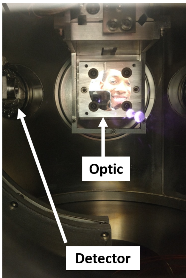
Figure 5.7: The optics section of the NIST SURF reflectometer. The detector is a Si-photodiode. The mirror sample was very shiny (in visible light) and smooth. So smooth, that we can see the author of this dissertation in the mirror.
