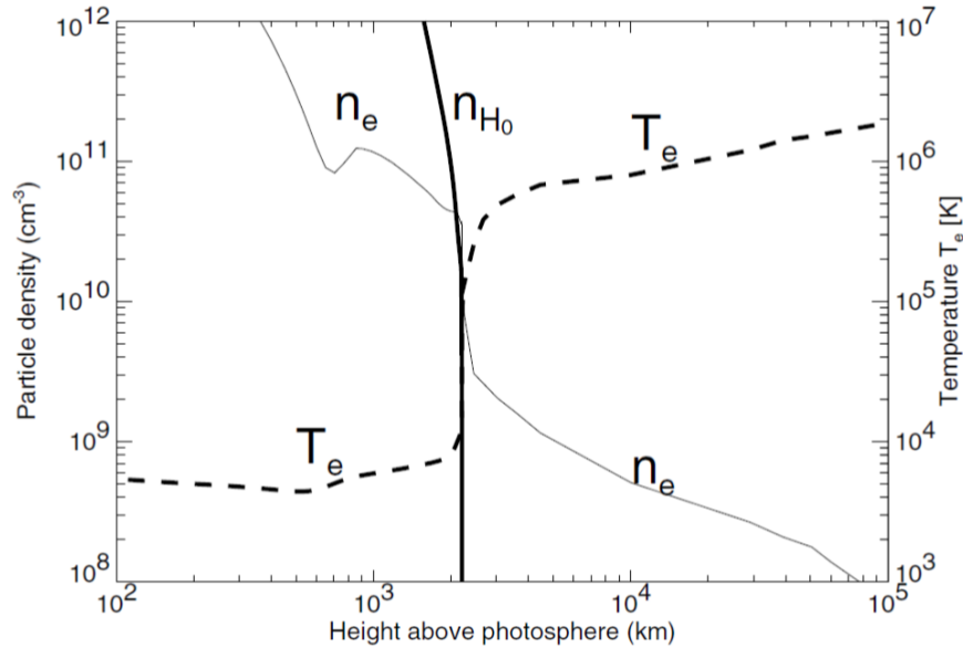
Figure 6.7: Approximated electron density and temperature as a function of height in the solar atmosphere. Figure adopted from [6].
