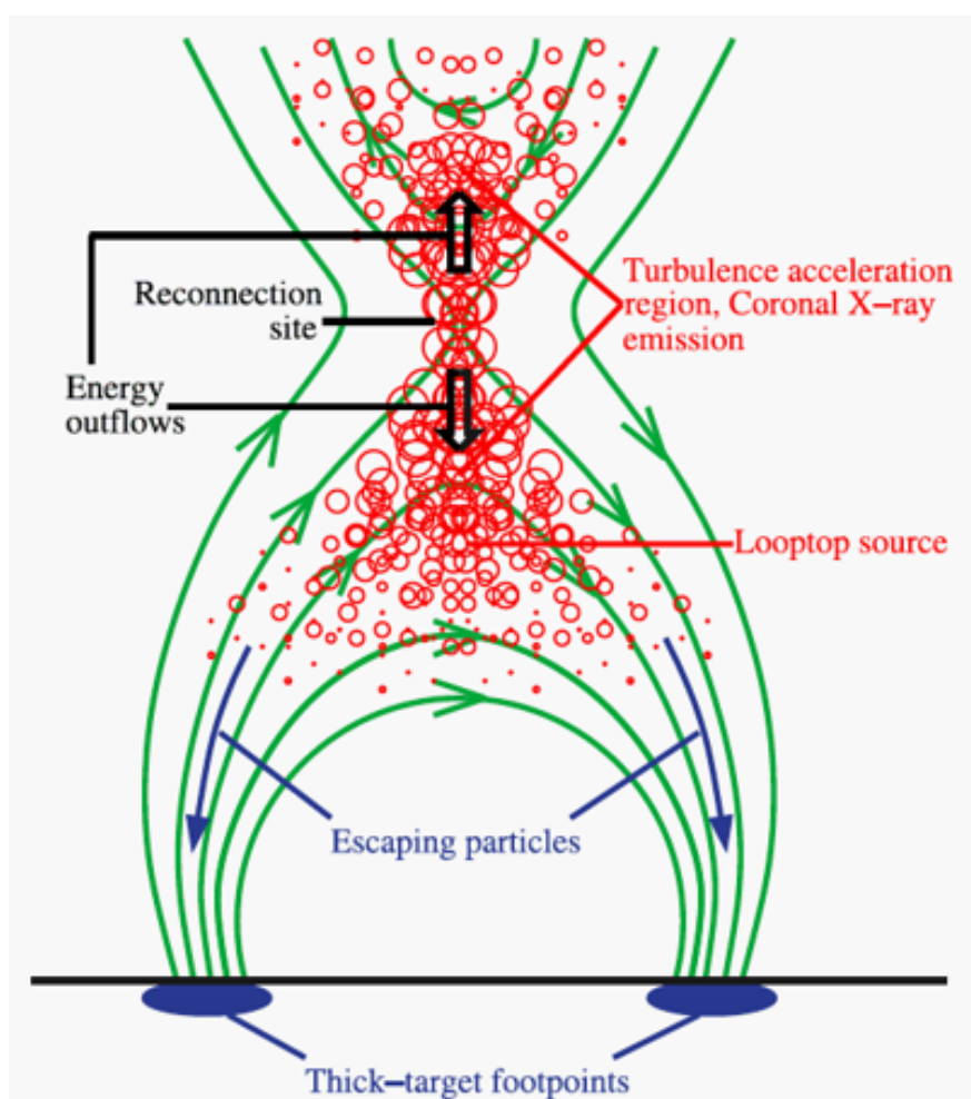
Figure 6.16: Diagram from Liu et al. 2008 [104] of possible reconnection set morphology for large solar flares. The green lines are the proposed magnetic field arrangement, red circles indicate possible turbulence, the blue disc would be the hard X-ray flare footpoint sources.
