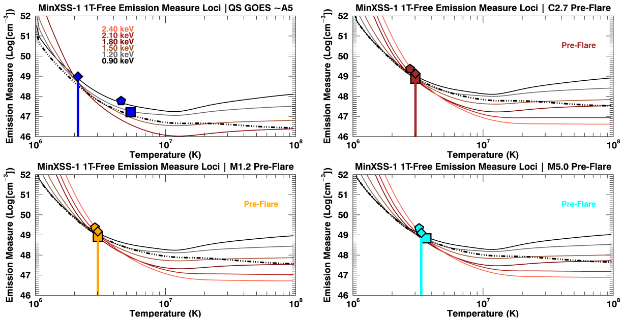
Figure 9.10: Volume emission measure loci (em loci) plots with MinXSS-1 OSPEX 1TFree fit parameters over-plotted as delta functions in temperature with filled diamonds indicating the emission measure value for the non-large-flaring sun (pre-flare). These MinXSS-1 em loci and fit parameters correspond to the spatial distribution captured by Hinode XRT in Figure 9.15. The solid colored lines correspond to X123 counts summed to 0.3 keV wide energy bins and the dash-dotted lines are the XP loci. The rainbow keV values in the top left plot indicate the color code for the minimum energy bin use for each X123 em loci. The em loci indicate the maximum emission if all the plasma was isothermal for each summed energy bins. GOES averaged values are listed for photospheric (pentagon) and coronal (square) abundances. The plot of X123 1TFree fits are to demonstrate, 1) the agreement with the overlapping X123 em loci, 2) agreement with the overlapping XP em loci and 3) consistency with the GOES XRS isothermal estimation except for low GOES levels like the \sim A5 levels (due to the non-linearity of GOES for low flux levels).
