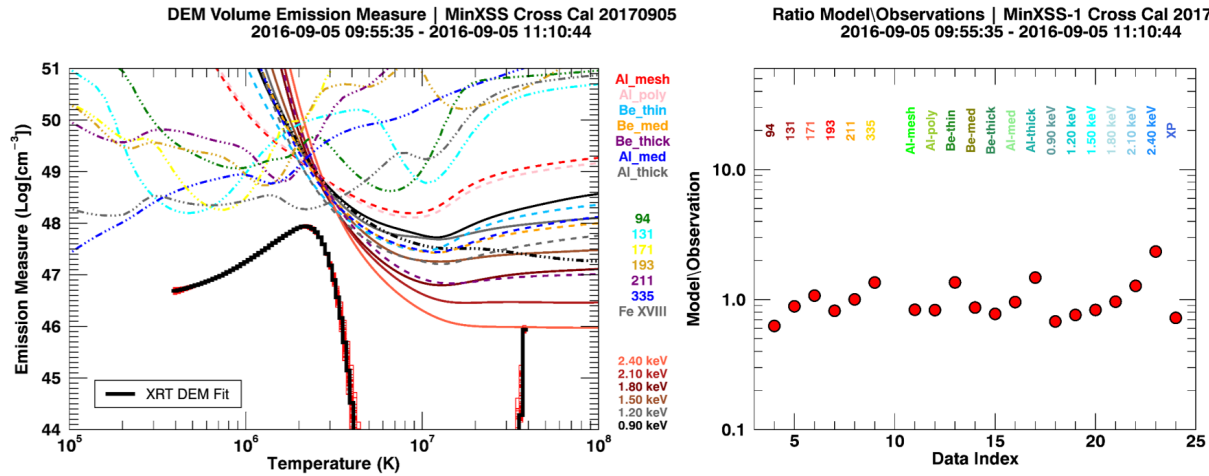
Figure 9.37: MinXSS-1 \leftrightarrow XRT cross-calibration on 2016 September 5. Left plot: MinXSS-1, XRT and AIA DEM fit results. VEM vs. temperature using the XIT method (black thick histogram line). The thin red histogram lines are 100 Monte-Carlo realizations and give an indication of the fit uncertainty. The uncertainty in the DEM has diminished drastically. The DEM is strongly constrained over the fit temperature range. AIA greatly improves the cool plasma inference. Right plot: MinXSS-1 X123 measured and DEM count rates.
