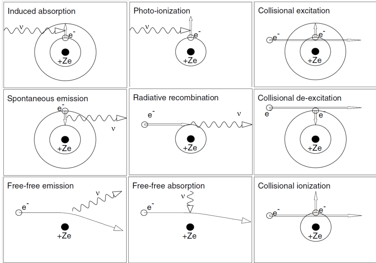
Figure 2.3: A subset of atomic processes relevant for the study in this dissertation. Adopted from Aschwanden 2005 [6].
