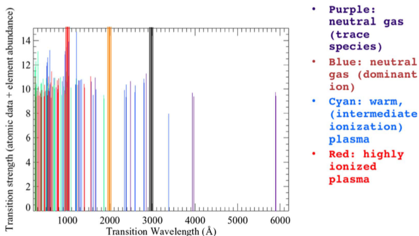
Figure 2.6: The number of relevant resonance lines for astrophysical investigations in general increases into the FUV and LUV. Below 1,000 Å is the highest density. Adapted from [141]
