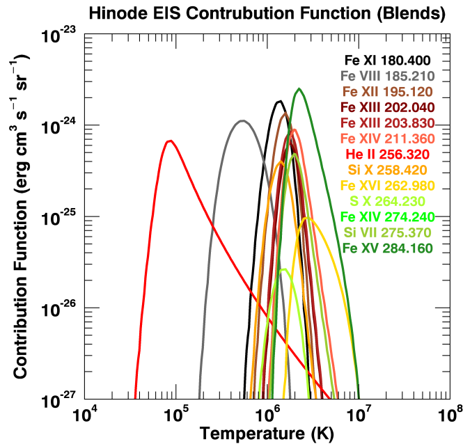
Figure 9.39: Example of the Hinode EIS line contribution functions G(T, E_{ij}, n_e) , ( \text{erg s}^{-1} \text{cm}^3 \text{sr}^{-1} ) using the nominal ‘coronal’ abundance and electron number density of 10^9 \text{cm}^{-3} . A huge difference between EIS and the broadband spectrometers or filter images that have been discussed thus far is that the temperature response for the EIS lines are much more centralized in temperature. The 40” slot data has a lower spectral resolution and thus there can be blends in each spectrally integrated EIS 40” slot image.
