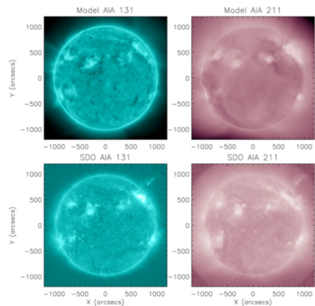
Figure 12.6: Comparison of AWSom synthesized EUV and AIA images. The figure is adapted from van der Holst et al. 2014 [151].
