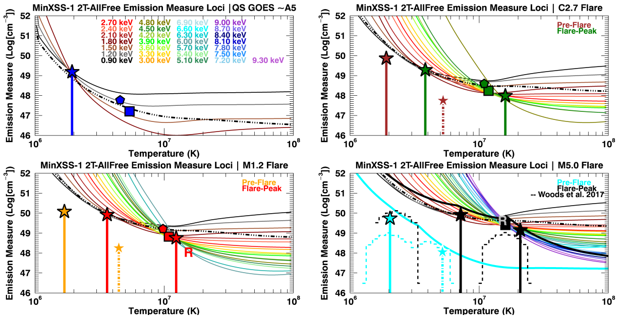
Figure 9.11: Em loci plots with MinXSS-1 OSPEX 2TAllFree fit flare-peak and QS parameters over-plotted as delta functions in temperature with filled stars indicating the emission emission measure value. The solid line delta functions are well constrained by the MinXSS data. The pre-flare dash-dot delta function without the black outline indicates that the hotter-dimmer component is less constrained by MinXSS data. The thin solid colored lines correspond to X123 counts summed to 0.3 keV wide energy bins and the dash-dotted lines are the XP loci. The rainbow keV values in the top left plot indicate the color code for the minimum energy bin use for each X123 em loci. The X123 and XP em loci are consistent. The [158] M5.0 flare fit results are overlaid as the dashed histograms in the bottom right panel. The thick black em loci is for the M5.0 flare and the thick cyan em loci for the pre-flare, both are the minimum of all the individual energy bins corresponding to the spectral model used in the [158] analysis. GOES averaged values are listed for photospheric (pentagon) and coronal (square) abundances. RHESSI values for the M1.2 and M5.0 flare are indicated by the ‘R’.
