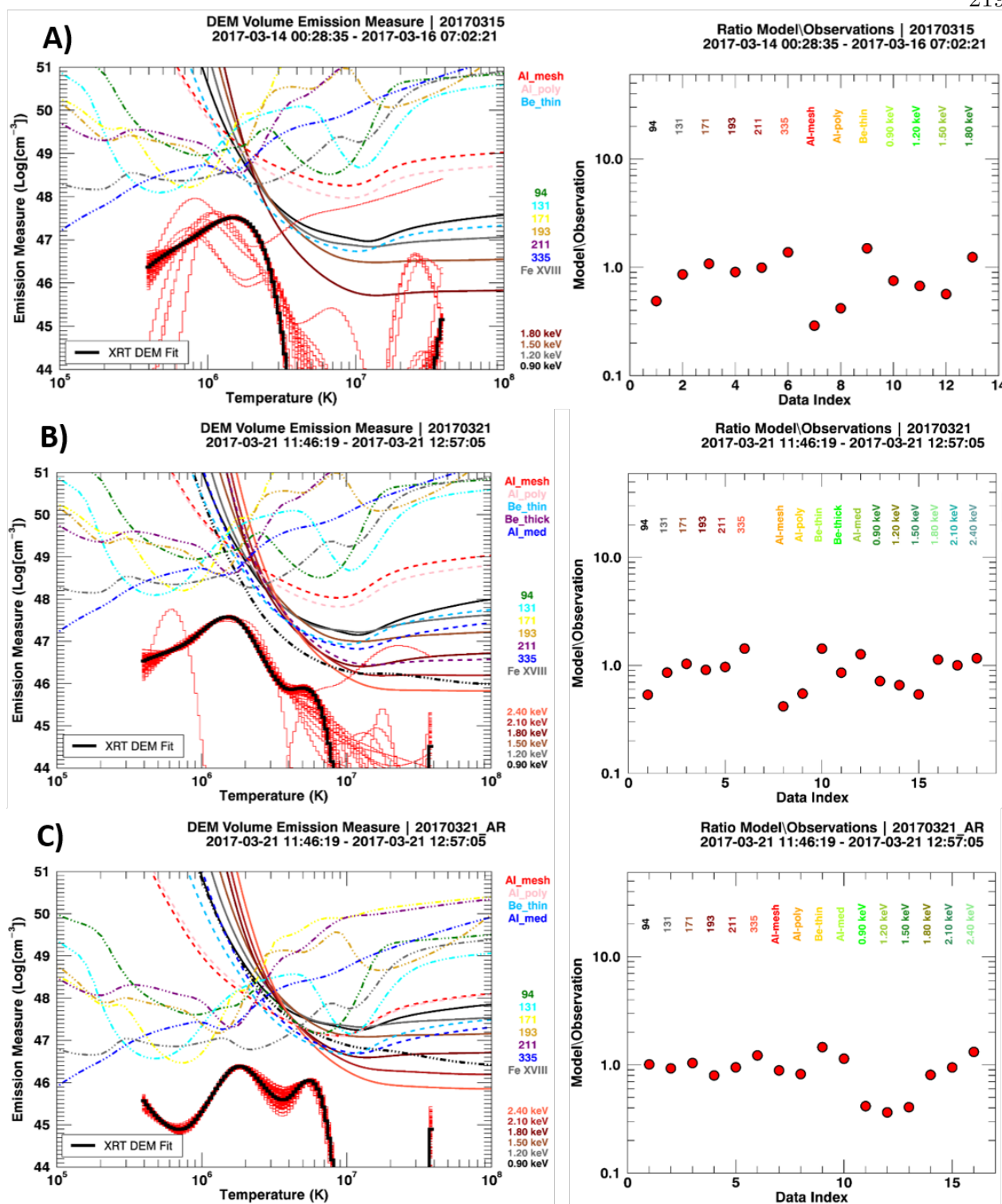
Figure 10.7: MinXSS-1, XRT and AIA combined DEM during ‘quiescent’ times (A) centered on 2017 March 15, time with an active region (B) on 2017 March 21, and the contribution from that same active region extracted (C). DEM predicted count rates are within roughly a factor of two for all data sets except Al-mesh and Al-poly in (A) and (b). The QS DEM peaks between 1 - 2 MK, which is common for the quiet Sun in the absence of active regions or large flares. The amount of plasma radiating for T \geq 2 MK drops precipitously. The AR DEM has significant contributions up to T \approx 7 MK
