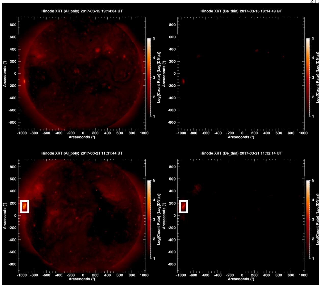
Figure 10.4: Top Row: QS Hinode XRT Al-poly (left) and Be-thin (right) Log-count rate images. Bottom Row: AR Hinode XRT observation with Al-poly (left) and Be-thin (right) images. The white box indicates the location of the AR that has rotated into the line of sight.
