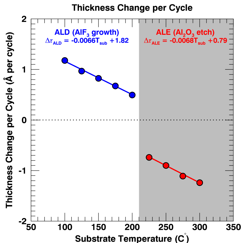
Figure 4.4: Thickness change per cycle in angstroms \text{\AA} , as a function of substrate temperature. The ALE of \text{Al}_2\text{O}_3 (red) and the ALD of \text{AlF}_3 (blue) temperature regime data are the symbols and the linear fits are the lines. The offset difference is primarily due to the LiF pre-conditioning in the ALE process, but the tcpc are very similar. ALD data is from Hennessy et al. 2016A [75] and ALE data is from Hennessy et al. 2017 [76].
