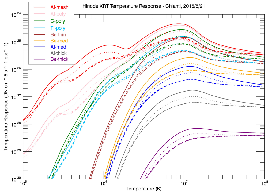
Figure 9.17: Example of the Hinode XRT filter temperature responses, F(T) , ( \text{DN s}^{-1} \text{cm}^5 \text{pixel}^{-1} ) in column emission measure units (CEM) for various abundances. The solid line is the nominal ‘coronal’ abundances of Feldman 1992 ( A_{low-fip} \approx 3 - 4 ), the dotted line is for the ‘Hybrid’ abundances from Schmelz et al. 2012 ( A_{low-fip} \approx 2 ), the dashed and dash-dot lines are for the photospheric derived abundances from Caffau et al. 2011 and Asplund et al. 2009 respectively ( A_{low-fip} = 1 ). It is obvious in the XRT temperature response curves, like the MinXSS curves that the X-ray emission is very sensitive to the elemental abundances of the emitting plasma.
