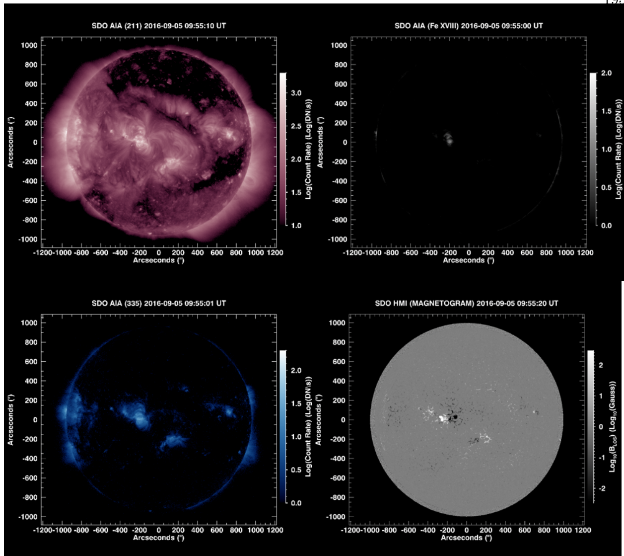
Figure 9.35: Log-scaled count rate AIA 211Å, 335Å, Fe XVIII and HMI images on 2016 September 5.
