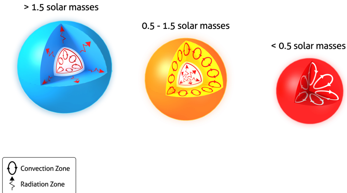
Figure 6.2: Stars with masses less than roughly 0.5M_{\odot} have fully convective interiors. Stars with 0.5M_{\odot} \leq M \leq 1.5M_{\odot} have a radiative inner portion and a convective outer portion. The most massive stars ( M > 1.5M_{\odot} ) have a convective inner portion and a radiative outer portion. The dynamics of the energy transport inside of stars have direct and profound implications on the atmospheric structure. Source: https://commons.wikimedia.org/wiki/File:Heat_Transfer_in_Stars.png under the Creative Commons Attribution-Share Alike 3.0 Unported License ( https://creativecommons.org/licenses/by-sa/3.0/deed.en )
