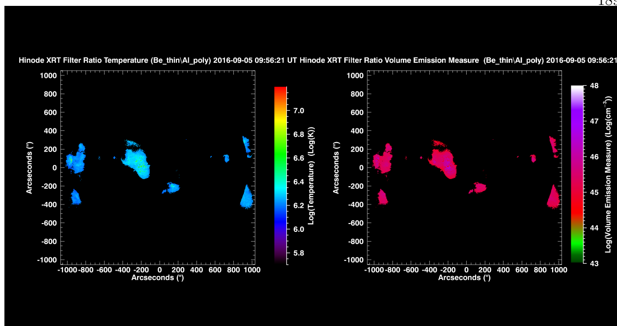
Figure 9.29: MinXSS-1 \leftrightarrow XRT cross-calibration on 2016 September 5. Left plot: XRT Be-thin and Al-poly filter ratio temperature map. Each pixel is assumed to be isothermal in this filter ratio formulation. Right plot: XRT Be-thin and Al-poly filter ratio VEM map.
