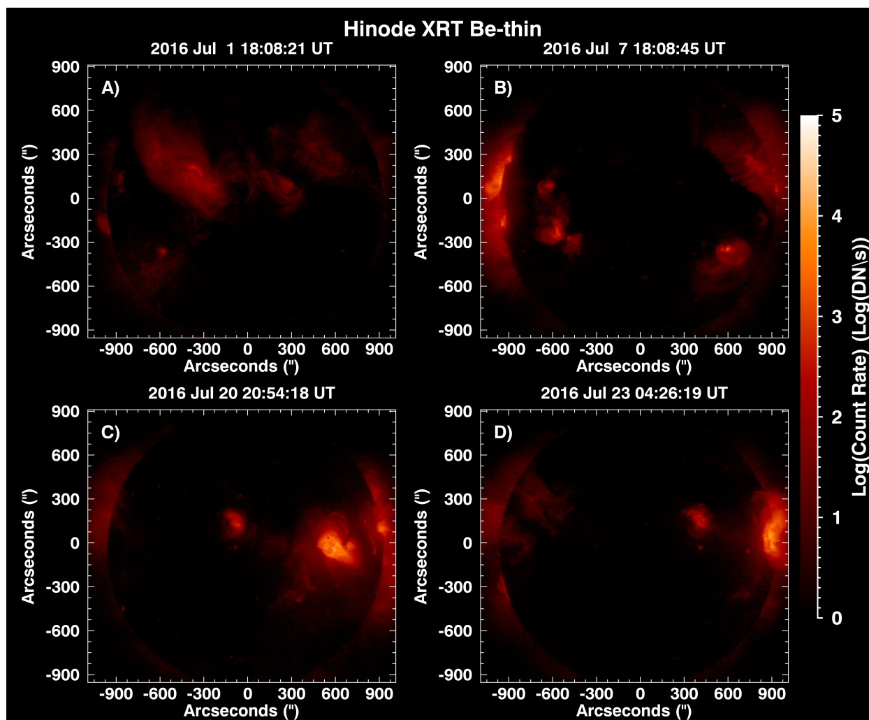
Figure 9.15: Log-scaled count rate Hinode X-ray Telescope (XRT) Be-thin full Sun images near the time of the MinXSS-1 observed QS (Panel A), Pre-flare times for the C2.7 (Panel B), M1.2 (Panel C) and M5.0 (Panel D) flares. The XRT images provide information on the spatial distribution of the soft X-ray emitting plasma, since MinXSS measurements are integrated across the entire FOV.
