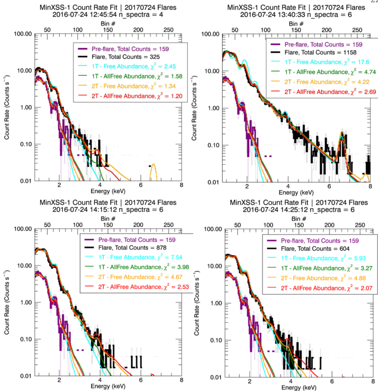
Figure 11.2: OSPEX Fits of the B and C class flares on 2016 July 24. The 1TFree fits are cyan, the 1TAllFree are green, the 2TFree are orange and the 2TAllFree are Red. The 2TAllFree are the best fits (lowest \chi^2_{reduced} ) of all the models.
