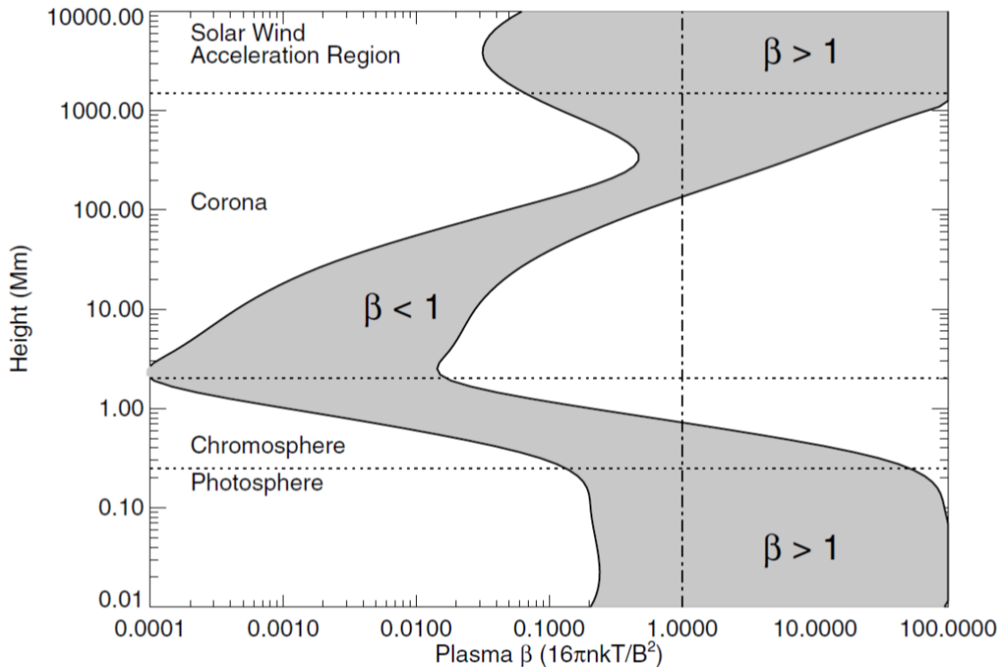
Figure 6.8: Plasma beta ( \beta = \frac{P_{gas}}{P_{magnetic}} ) as a function of height in the solar atmosphere. Image credit [6, 52]. The plasma beta is large in the photosphere (gas dominates the dynamics), smaller in the corona (magnetic field dominates dynamics) and large again in in the solar wind.
