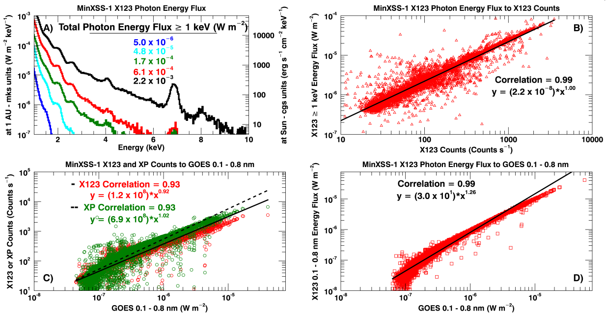
Figure 9.8: Panel A shows the MinXSS-1 X123 derived photon energy flux at 1 AU (in mks units - \text{W m}^{-2} \text{ keV}^{-1} ) and scaled back to the Solar surface (in cgs units - \text{erg s}^{-1} \text{ cm}^{-2} \text{ keV}^{-1} ). The total energy flux at 1 AU as measured by MinXSS-1 for photon energies \geq 1 \text{ keV} is listed for the GOES \sim A5 (blue), B5 (cyan), C2.7 (green), M1.2 (red) and M5.0 (black) class observations. Panels B - D contain scatter plots, correlation coefficients and linear fit of MinXSS-1 X123 photon energy \geq 1 \text{ keV} to count rate (Panel B), MinXSS-1 X123/XP count rate to GOES 0.1 - 0.8 nm flux (Panel C) and MinXSS-1 X123 photon energy flux integrated from 0.1 - 0.8 nm ( \sim 1.55 - 12.4 \text{ keV} ) to GOES XRS 0.1 - 0.8 nm flux (Panel D) all show very strong correlations, validating the MinXSS data.
