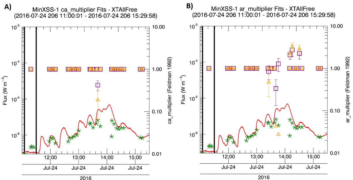
Figure 11.6: OSPEX XTAllFree abundance Fits for Ca (left) and Ar (right) of the flares on 2016 July 24. The 1T components are orange, the 2T components are purple (triangle and squares). Ca only has a few instances where the signal-to-noise ratio in the 4 keV spectral feature is large enough to allow the Ca abundance to be free. All that can be stated is that it is less than the Feldman 1992 values when allowed to be free. Ar is a high-fip element and shows an enhancement for some instances and a depression for others. Ar is known to have anomolous abundance effects durring flares [40, 39].
