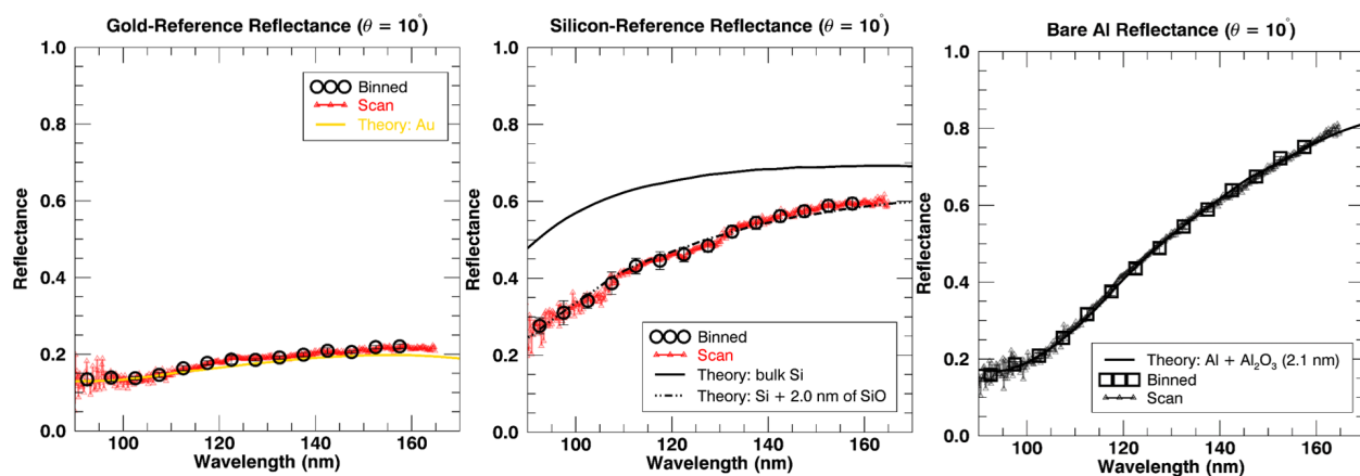
Figure 5.12: LASP CTE3 reflectance measurements of reference sample if gold (Au), silicon (Si) and bare aluminum with native oxide (Al). The yellow and black lines are calculations based upon optical constants. The red lines is the raw reflectance calculated from the ratio of the spectral scans. The symbols are the binned raw reflectance data.
