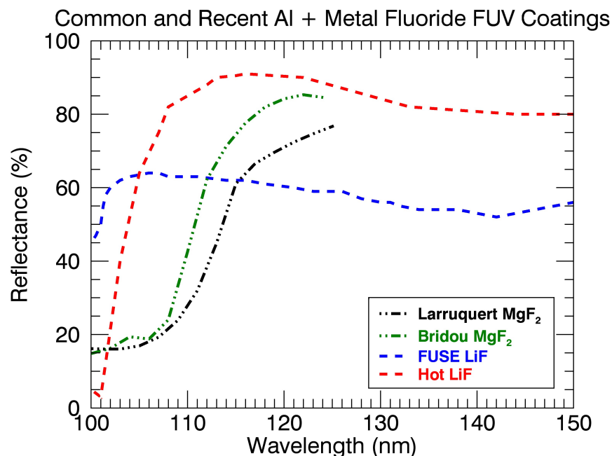
Figure 3.4: A non-exhaustive example of the current optical coatings of MgF 2 and (LiF) on Al. Adopted from Moore et al. 2016 [113].
