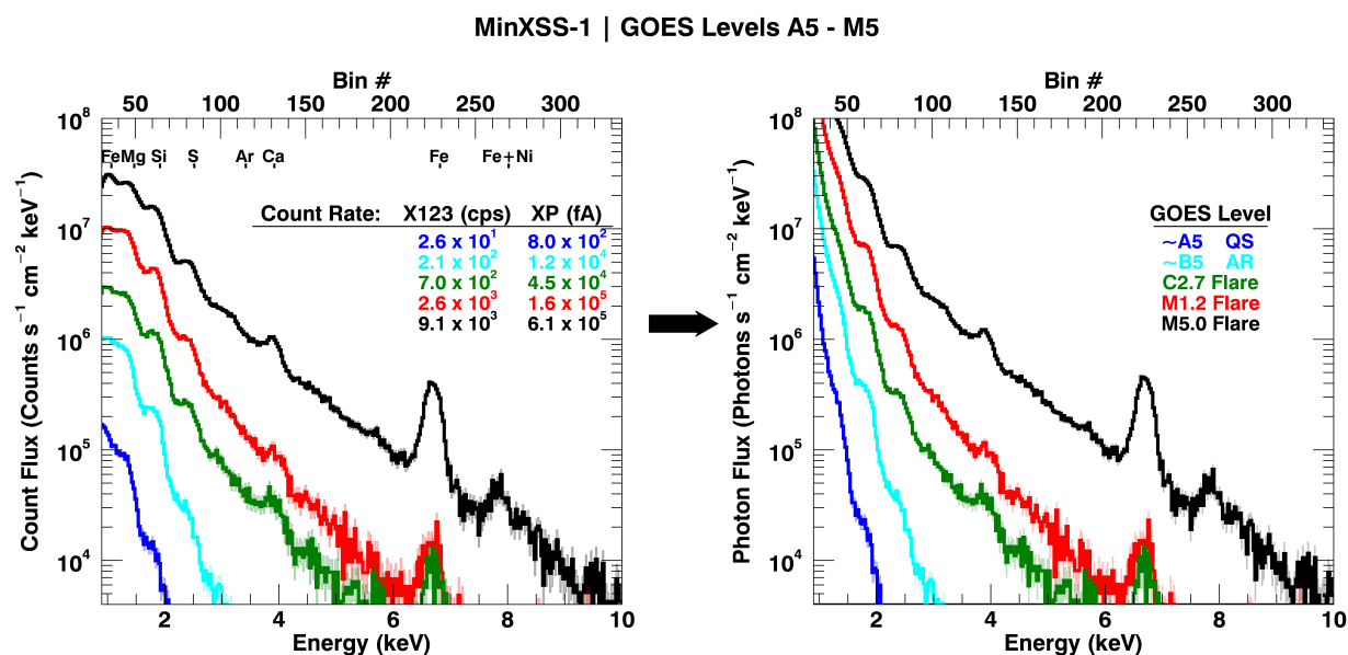
Figure 9.7: MinXSS-1 X123 solar measurements (solid lines) from GOES A5 to M5 levels ( \sim 5 \times 10^{-8} - 5 \times 10^{-5} \text{ W m}^{-2} ). The left plot is the mean count flux and the right plot is the estimated photon flux. The uncertainties are depicted as the shaded region around the measurements. This demonstrates the dynamic range of the MinXSS-1 spectrometer, and the variation in spectral features for increasing solar flux levels. The ‘bumps’ in the spectrum are due to groups of dominant emission lines from ionized Fe near 1.2 keV and 6.7 keV, Mg near 1.7 keV, Si around 2.1 keV, S by 2.7 keV, Ar (or lack thereof) near 3 keV, Ca by 4 keV, and the Fe+Ni complex at 8 keV. These features can be used as elemental abundance probes to assess deviations from the traditional ‘Coronal’ abundance values during various solar conditions.
