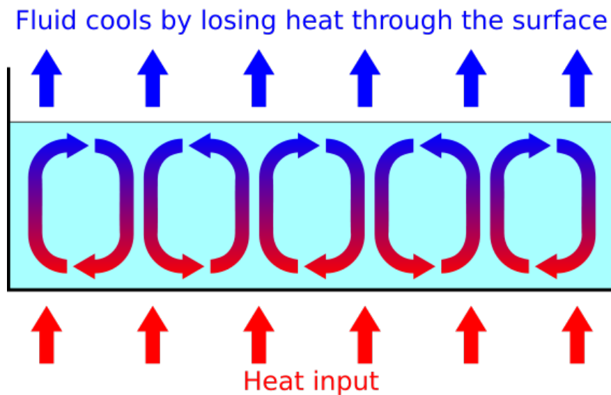
Figure 6.3: Convection transports energy by fluid motions. In gravitationally stratified convection, a hot parcel of material flows upwards due to buoyancy forces (adiabatic process), expands as it rises (pressure equilibrium), loses heat at the ‘surface’ (generally taken as a scale height), cools, and migrates downward, to be heated and return to rise. Source: https://commons.wikimedia.org/wiki/File:ConvectionCells.svg under the Creative Commons Attribution-Share Alike 3.0 Unported License ( https://creativecommons.org/licenses/by-sa/3.0/deed.en ).
