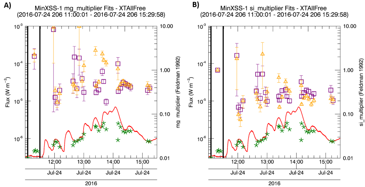
Figure 11.5: OSPEX XTAllFree abundance Fits for Mg (left) and Si (right) of the flares on 2016 July 24. The 1T components are orange, the 2T components are purple (triangle and squares). Mg abundance decreases during the flares and so does Si.
