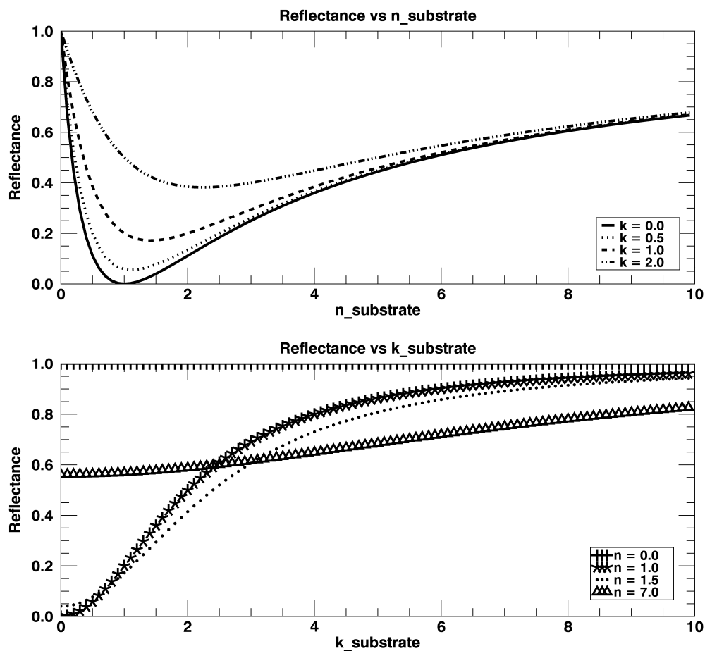
Figure A.2: Top Plot: Theoretical reflectance as a function of n vs. fixed k in air. For k = 0 and n = 1.0 , the reflectance vanishes because n = n_{air} . Bottom Plot: Theoretical reflectance as a function of k vs. fixed n in air. For n = 0 the reflectance is 100% for all k , because the numerator and the denominator are the same and cancel out when n = 0 .
