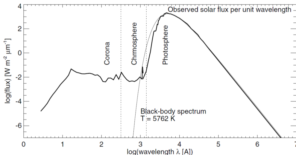
Figure 6.13: Composite spectral energy distribution (SED) from X-rays to infrared for the Sun. The majority of the visible light emission originates in the photosphere, the UV mostly created in the warmer chromosphere and X-rays (and EUV) are birthed, generally in the corona.
