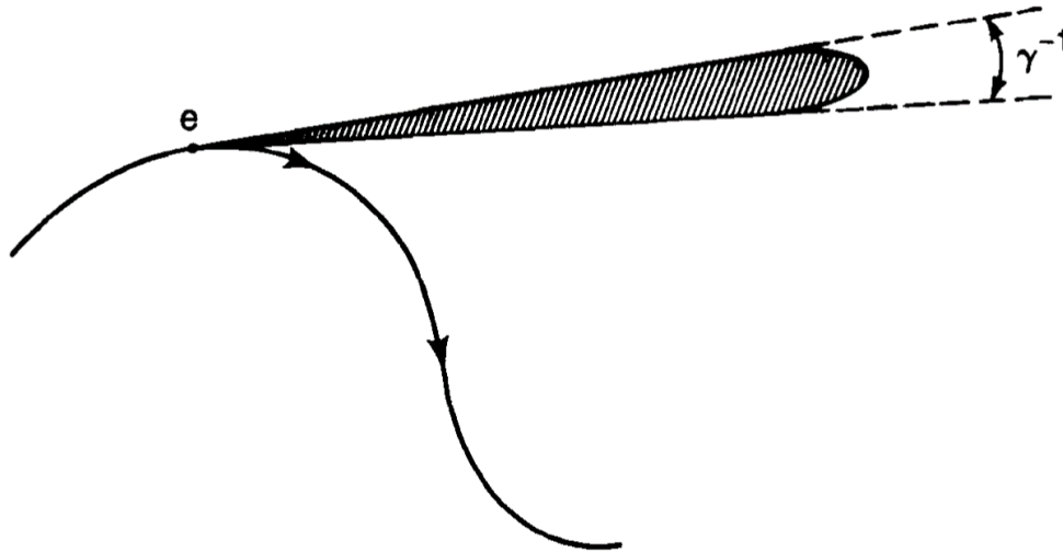
Figure 2.4: Diagram adopted from Kim 1989 [84] displaying the beamed radiation pattern of the accelerated electron, with velocity near the speed of light, traveling a curved path.
