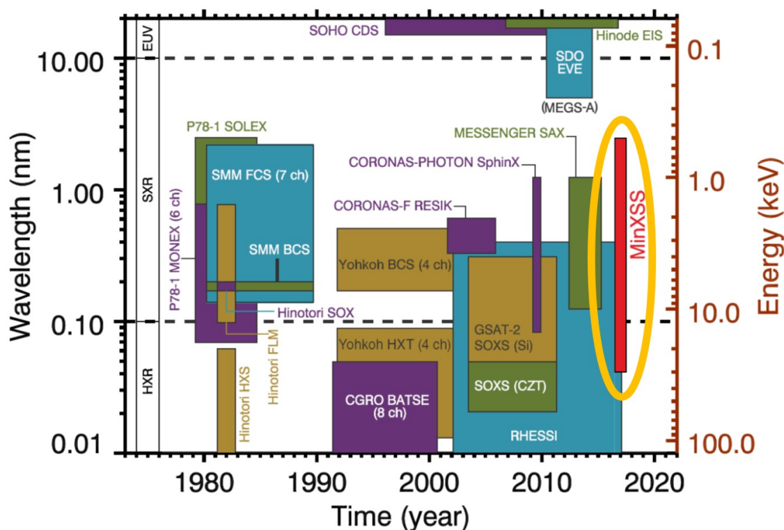
Figure 7.1: A non-exhaustive list of solar EUV and X-ray space borne instruments. The majority of soft X-ray missions conducted either high spectral resolution ( < 0.1 keV) measurements over a narrow bandpass, had fairly low spectral resolution ( > 1.0 keV) over a large spectral bandpass, or were integrating photometers. The MinXSS CubeSats will combine moderate spectral resolution ( \sim 0.15 keV FWHM at 5.9 keV) and a fairly large spectral bandpass (0.5 - 30 keV).
