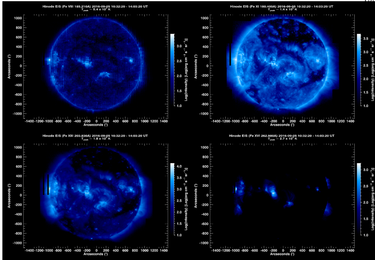
Figure 9.38: Log-scaled energy intensity ( \text{ergs cm}^{-2} \text{s}^{-1} \text{sr}^{-1} ) of Fe VIII ( 185.21 \text{ \AA} , T_{peak} \sim 5.4 \times 10^5 \text{ K} ), Fe XI ( 180.40 \text{ \AA} , T_{peak} \sim 1.4 \times 10^6 \text{ K} ), Fe XIII ( 203.83 \text{ \AA} , T_{peak} \sim 1.8 \times 10^6 \text{ K} ) and Fe XVI ( 262.98 \text{ \AA} , T_{peak} \sim 2.7 \times 10^6 \text{ K} ) images on 2016 September 5.
