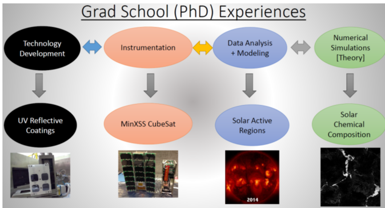
Figure 1.1: Diagram of a few main aspects of astrophysics: Technology Development, Instrumentation, Observations plus Data Analysis, and Numerical Simulations. The bottom rows illustrate the research included in this dissertation.
