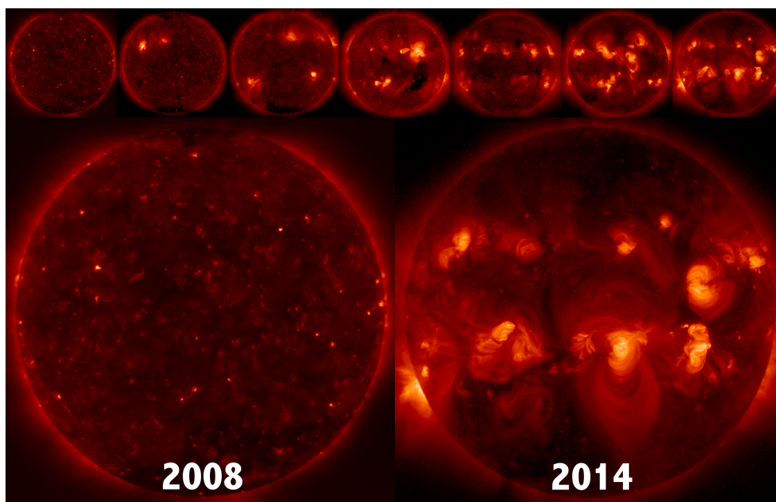
Figure 6.10: Hinode XRT images on 2008 and 2014. The change in the magnetic structure over the solar cycle is clear as the number of active regions (large scale magnetic structures) is much greater near the maximum of Solar Cycle 24. Image credit, the Hinode Team.
