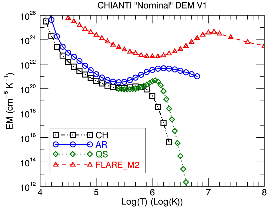
Figure 6.15: Differential Emission Measure (DEM) nominally stored in the CHIANTI Atomic Database. The coronal hole (black) is fairly void of plasma greater than 1 MK that is radiating, the quiet Sun (green) has the majority of the radiating plasma between 1 - 2 MK (except for the chromospheric contribution for T \leq 0.5 MK). Active regions (blue) have contributions from hotter plasma (3 - 5 MK) and solar flares (red) manifest the highest temperature plasma (well over 10 MK).
