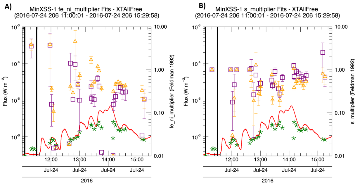
Figure 11.4: OSPEX XTAlFree abundance Fits for Fe, Ni (left) and S (right) of the flares on 2016 July 24. The 1T components are orange, the 2T components are purple (triangle and squares). Fe and Ni have enough signal to noise to be free for most times to allow the abundance to be free. In general, most of the values decrease during the flares. The same appears to be true for S.
