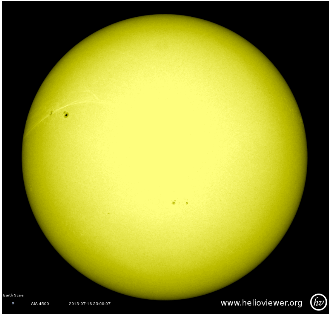
Figure 6.4: Visible light satellite image of the solar photosphere from the Solar Dynamics Observatory (SDO) and Atmospheric Imaging Assembly (AIA).
