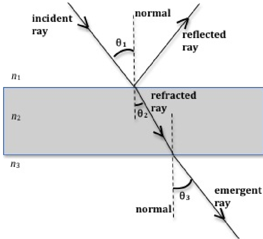
Figure A.1: Diagram describing the ray approximation of light propagation from medium with index of refraction, n_1 and angle of incidence, \theta_1 , the reflected angle from the normal, \theta_1 , in the secondary medium with, n_2 , and angle of propagation, \theta_2 , and a third medium with n_3 , and angle of propagation, \theta_3 . The plane in which the incident and reflected ray propagate is called the plane of incidence. Image credit: http://www.webassign.net/labsgraceperiod/ncsulcpem2/lab_6/manual.html .
