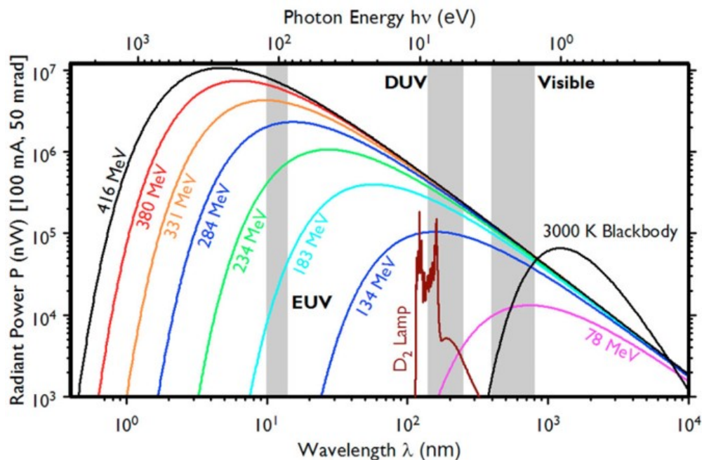
Figure 2.5: Example spectral flux as a function of the mean electron energy ( E_e ). The greater the electron energy the greater the photon flux at all photon wavelengths (energies). Synchrotron radiation spans large portions of the electromagnetic spectrum. Adapted from Arp et al. 2011 [5]
