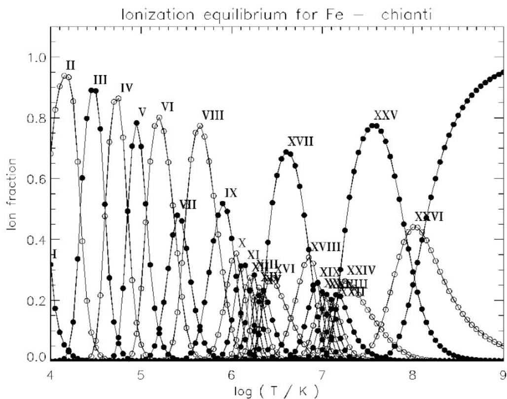
Figure 6.14: CHIANTI Atomic Database calculation of Fe ionization states as a function of temperature assuming collisional ionization equilibrium (CIE). The radiation from different ionization states can be used to probe the temperatures present in a plasma.
