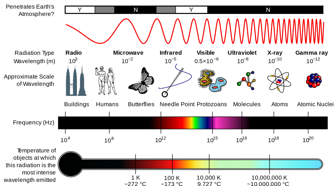
Figure 2.1: The electromagnetic spectrum is vast, spanning over 15 orders of magnitude in wavelength, frequency and energy space. Source: https://commons.wikimedia.org/wiki/File:EM_Spectrum_Properties_edit.svg under the Creative Commons Attribution-Share Alike 3.0 Unported License ( https://creativecommons.org/licenses/by-sa/3.0/deed.en ).
