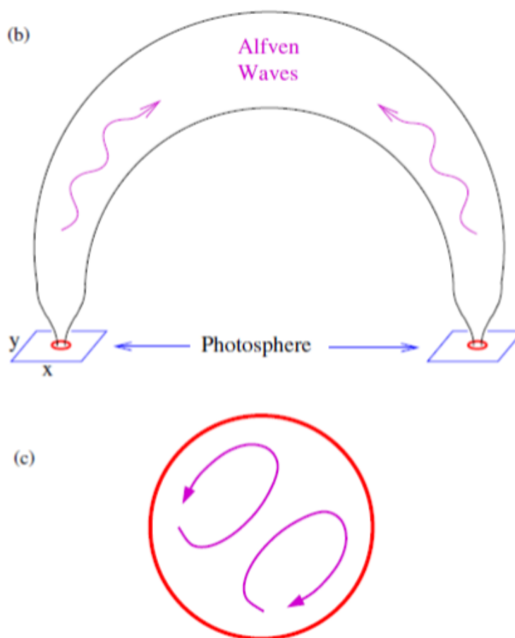
Figure 6.12: (b) Diagram of alfvén wave propagation in magnetic loops from van Ballegoijen et al. 2014 [149]. (c) proposed velocity motions inside of magnetic flux elements.
