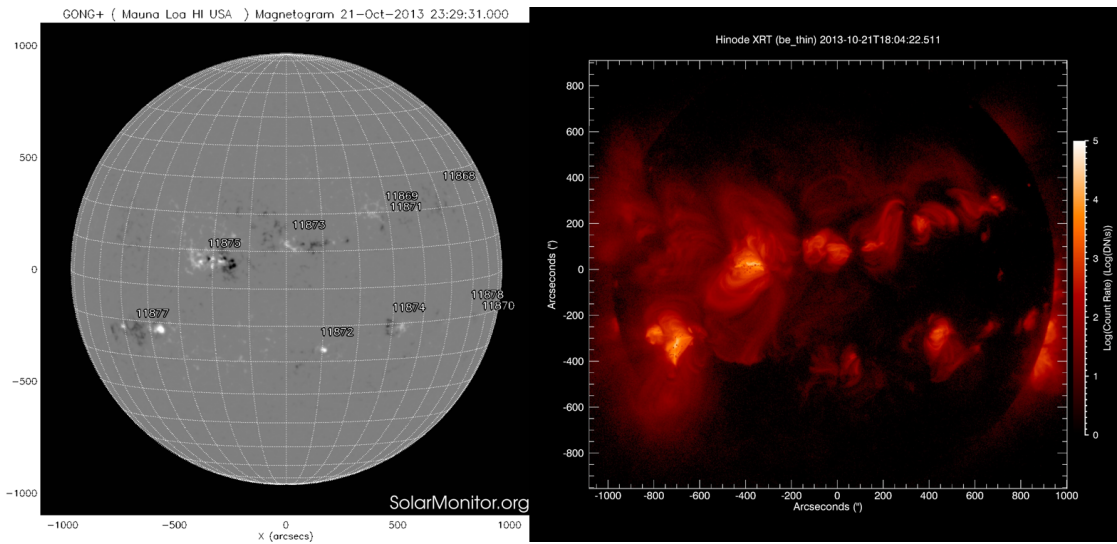
Figure 6.9: Left panel: GONG line-of-sight magnetogram showing the locations of sunspots on 2013 October 21. Right panel: Hinode XRT observations displaying active regions on 2013 October 21. It is apparent that the sunspots and active regions are co-spatial and originate from the same phenomena, magnetic fields.
