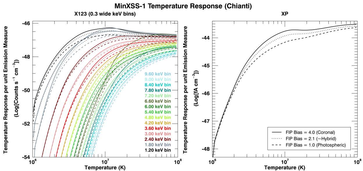
Figure 9.1: An example of the X123 and XP temperature response functions for a spectrum summed to 0.3 keV wide bins for X123 (ten 0.03 native bins). The temperature response is in volume emission measure units of \text{cm}^{-3} . The isothermal spectral emission model used to compute the spectral response of the MinXSS instruments per plasma temperature is a spectrally extended version of the SolarSoftware (SSW) f_vth function (which uses the Chianti Atomic Database). The temperature response in soft X-rays can vary due to differences in the abundance of the low-FIP elements of Fe, Mg, Si, Ca and the mid-FIP element S used in the spectral emission model. Thus, we display the temperature response for traditional ‘Coronal’ [48] (4 times photospheric for the low-FIP elements), ‘Hybrid’ [138] ( \sim 2.1 times photospheric), and one of the latest photospheric [23] abundances. The MinXSS instrument temperature response begins to deviate for different abundances for plasma temperatures greater than 2 MK, due to the ions of the low-FIP elements.
