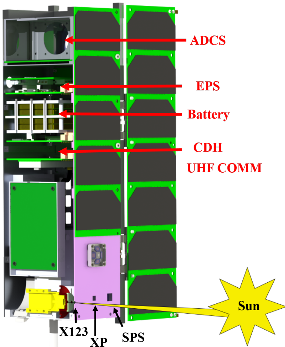
Figure 7.4: Cut out of the MinXSS CubeSat to demonstrate the optical path of the Sun (not to scale) through the field of view limiting aperture and housing for the X123 spectrometer. The X123, XP and SPS apertures, and other subsystem locations are labeled for clarity.
