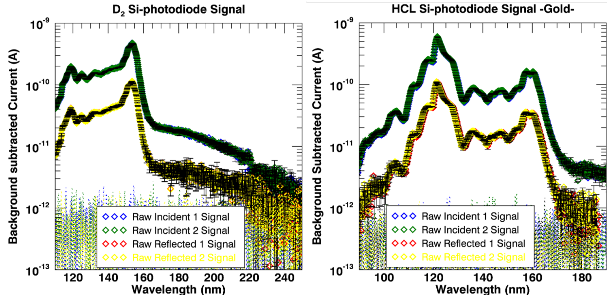
Figure 5.11: LASP CTE3 D 2 and HCL (H/Ar) light source spectral scan with the Si-photodiode. The input ( I_0 ) and reflected ( I_r ) signal is large enough for reflectance calculations with moderate signal-to-noise ( S/N \geq 5 ). There are two sets of spectral scans and they agree very well. The ratio of this example raw signal is used for the reflectance measurement result.
