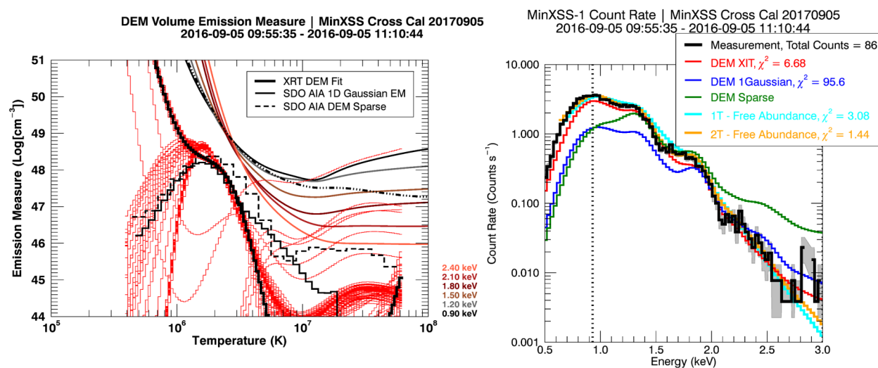
Figure 9.14: MinXSS-1 \leftrightarrow XRT cross-calibration on 2016 September 5. Left plot: MinXSS-1 XP and X123 only DEM fit results. VEM vs. temperature using the XIT method (black thick histogram line). The thin red histogram lines are 100 Monte-Carlo realizations and give an indication of the fit uncertainty. The XIT DEM is from the spatially integrated MinXSS-1 data. The thin black histogram line is the 1 Gaussian DEM result using AIA data only. The thin black histogram dashed line is the Sparse DEM result using AIA data only. The AIA only DEMs will be discussed in detail in the AIA calibration section. Both AIA only DEMs have substantial very hot plasma ( T \geq 10 MK) inference that over estimate the observed X123 count rates. The 1 Gaussian and Sparse DEM are solved per pixel grouping and averaged over the positive pixels. The colored solid lines are the X123 em loci and the dash-dot-dot-dot black line is the XP em loci. Right plot: MinXSS-1 X123 measured and DEM count rates. The XIT predicted MinXSS-1 count rates agree very well given all the uncertainties in the DEM fitting process.
