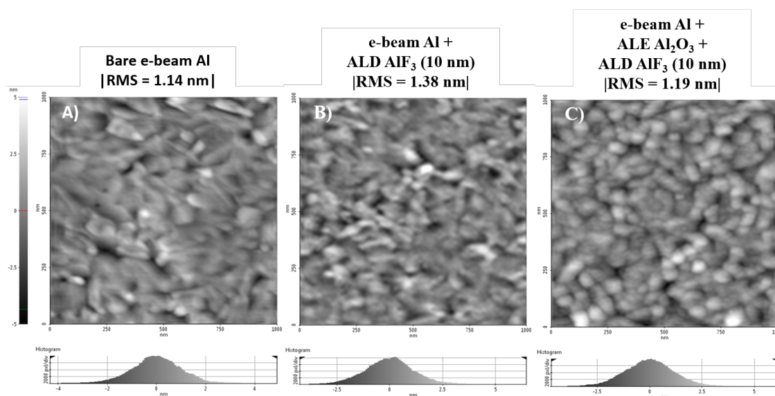
Figure 4.8: Atomic force microscopy (AFM) profile of surface roughness. The ALD of \text{AlF}_3 increases the surface roughness (as expected). The ALE of \text{Al}_2\text{O}_3 maintains a smooth surface which is beneficial for UV reflectance.
