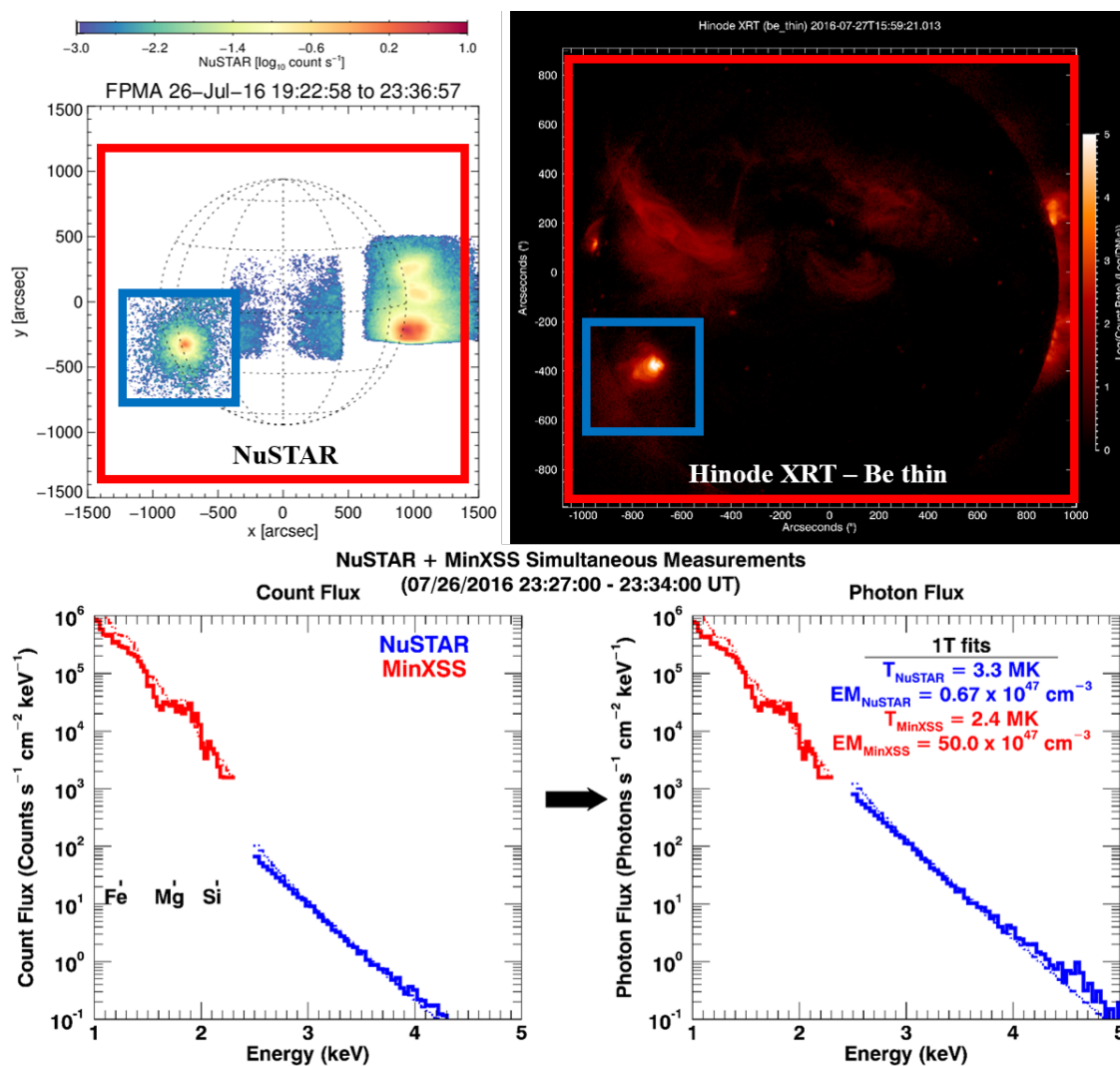
Figure 12.5: Top Left: Previous NuSTAR solar measurement. Top Right: Closest time Hinode XRT Be-thin image to the NuSTAR measurement. The blue (red) box indicates the spatial region that the NuSTAR (MinXSS) measurements (solid lines), inferred photon flux and 1T fit results (dash-dot lines). The emission measure (EM) is listed in volume units ( \text{cm}^3 ).
