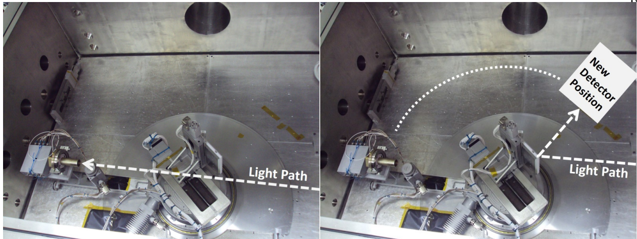
Figure 5.1: Inside the CASA Square Tank chamber. A microchannel plate detector is used from 90 - 130 nm and a photomultiplier tube with a \text{MgF}_2 window for wavelengths between 120 - \sim 300 nm. The left picture shows the detector position for the input light measurement ( I_0 ) and the right plot the position for reflected light measurement ( I_r ).
