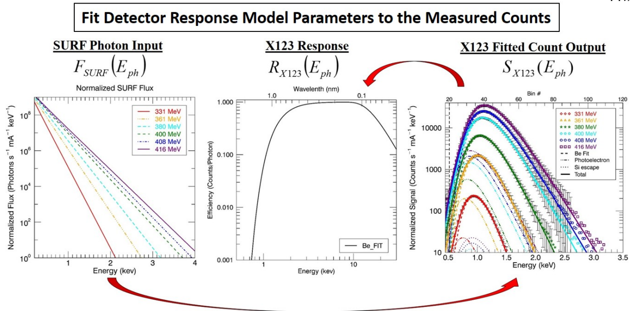
Figure 8.6: Outline of NIST SURF Multienergy technique to estimate the X123 spectral response. We fit a model of detector response parameters to the measured count flux from the SURF photon flux. Fitting the measured counts over the 0.5 - \sim 3.0 keV spectral range allows us to estimate the entire spectral efficiency from 0.5 - 30 keV from the model parameters. The main fit parameter is the Be window thickness. Other subsidiary components include contributions from escape of Si fluorescence photons from K and L (2s and 2p) excitations and photoelectrons produced in the Be window.
