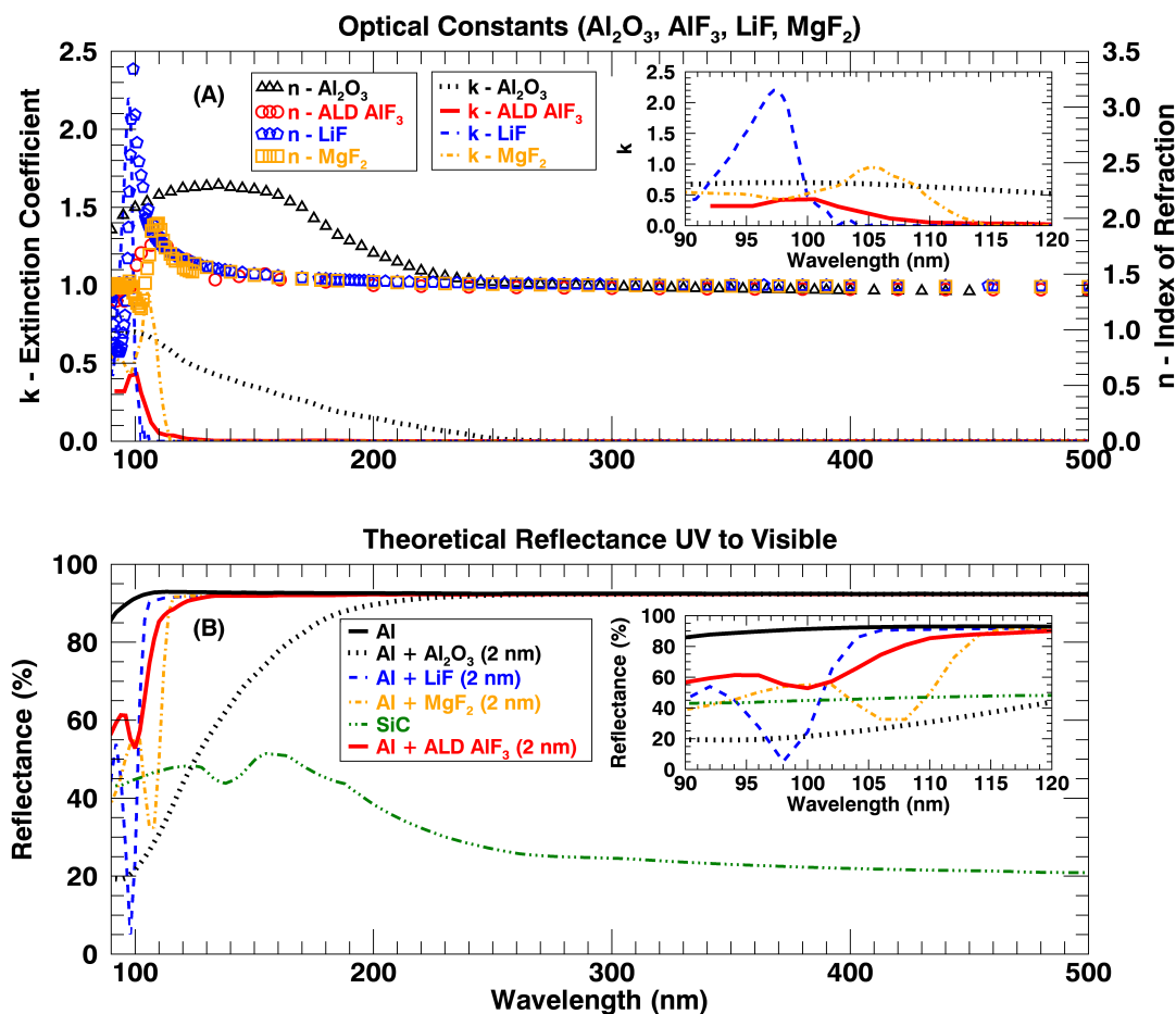
Figure 3.1: (A) Optical Constants from 90 - 500 nm for \text{Al}_2\text{O}_3 , \text{AlF}_3 , \text{LiF} and \text{MgF}_2 . The insert is only the extinction coefficient from 90 - 120 nm. \text{Al}_2\text{O}_3 has substantial absorption below 250 nm, \text{AlF}_3 has moderate absorption below 107 nm, \text{LiF} has strong absorption below 102 nm and \text{MgF}_2 is absorbing below 115 nm. (B) Reflectance calculations from 90 - 500 nm based on optical constants for Al + \text{Al}_2\text{O}_3 , Al + \text{AlF}_3 , Al + \text{LiF} , Al + \text{MgF}_2 (all 2 nm thick) and SiC. The insert is from 90 - 120 nm and demonstrates that ALD \text{AlF}_3 has the highest average reflectance in this wavelength range. The inverse relation between the extinction coefficient, k , and reflectance is apparent
