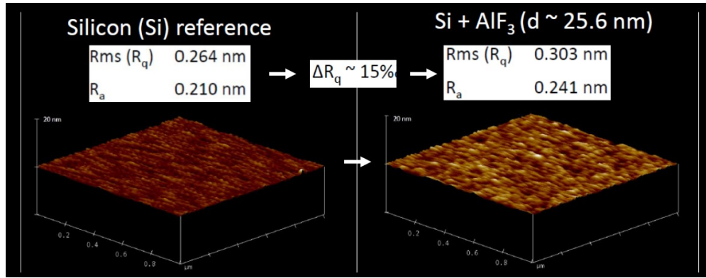
Figure 4.5: Atomic force microscopy (AFM) profile of surface roughness comparing a bare Si wafer and ALD of AlF_3 of \sim 25.6 nm. The ALD AlF_3 only increases the wafer surface roughness by \sim 15\% at an absolute thickness value of 0.303 nm root-mean-square (RMS). RMS = R_q = \sqrt{\frac{1}{n}(\sum_{i=1}^n z_i^2)} and the arithmetic average roughness, R_a = \sqrt{\frac{1}{n}(\sum_{i=1}^n |z_i|)} . Which is much smaller than the lowest wavelengths (90 nm) of the designed usage. Figure adapted from Moore et al. 2015 [114].
