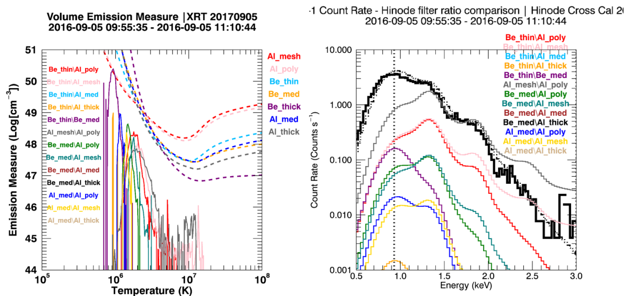
Figure 9.30: MinXSS-1 \leftrightarrow XRT cross-calibration on 2016 September 5. Left plot: VEM vs temperature distribution for various XRT filter ratios. Different ratios emphasize different temperature ranges. Right plot: MinXSS-1 X123 measurements (black histogram) and XRT filter ratio predictions (color histograms). None of the XRT filter ratios can recreate the X123 spectrum. This is expected because the Sun is not isothermal.
