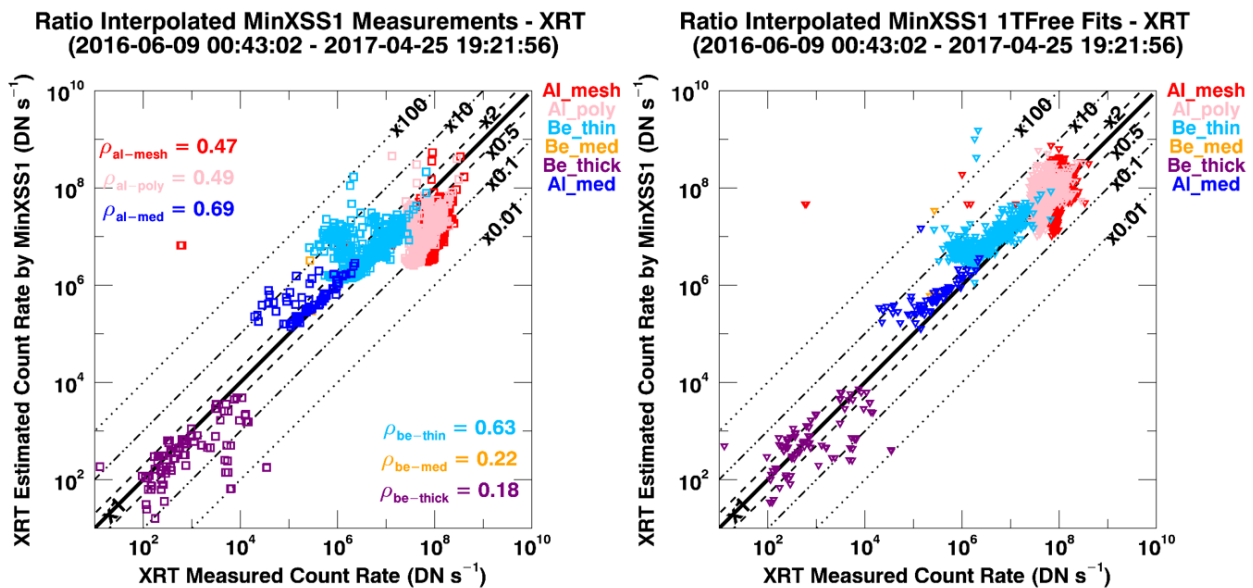
Figure 9.19: MinXSS-1 X123 estimated XRT count rate from the 15 minute averaged data interpolated to the XRT synoptic time frame. The Be-thin and Al-med are the most consistent for the actual X123 data (left) and the OSPEX 1TFree fit (right).
