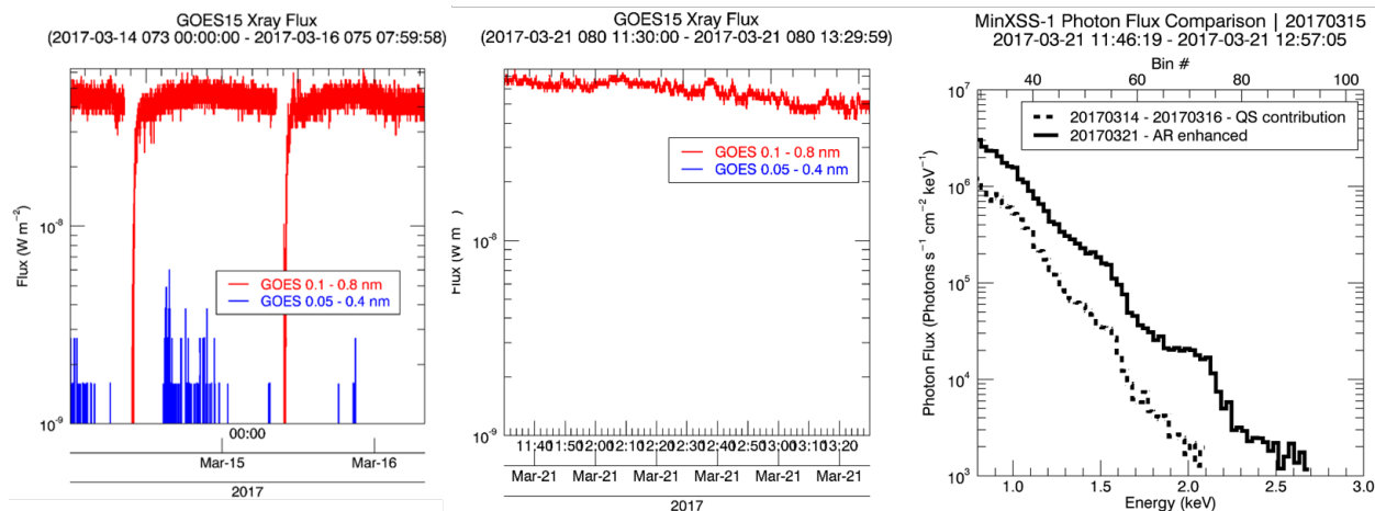
Figure 10.1: GOES 0.1 - 0.8 nm (red) and 0.05 - 0.4 nm (blue) energy fluxes vs. time for the QS extraction (2017 March 14 - 16, GOES \sim A4) and the AR contribution estimation (2017 March 21, GOES \sim A6). The Sun was very ‘quiet’. Middle plot: Right plot: X123 directly derived (‘inverted’) photon flux incident on the X123 aperture.
