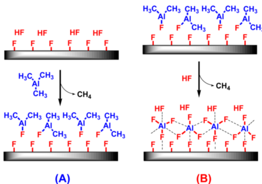
Figure 4.3: ALD of \text{AlF}_3 using hydrogen fluoride (HF) and trimethylaluminum (TMA) for the F and Al containing precursor gases respectively. Subsequent exposure of the precursor gases can lead to self-limiting, near stoichiometric mono-layer growth, providing a precise thickness-change-per-cycle for ideal conditions. Cyclic exposure of the precursors leads to steady conformal film growth. Figure adapted from Lee et al. 2015 [97].
