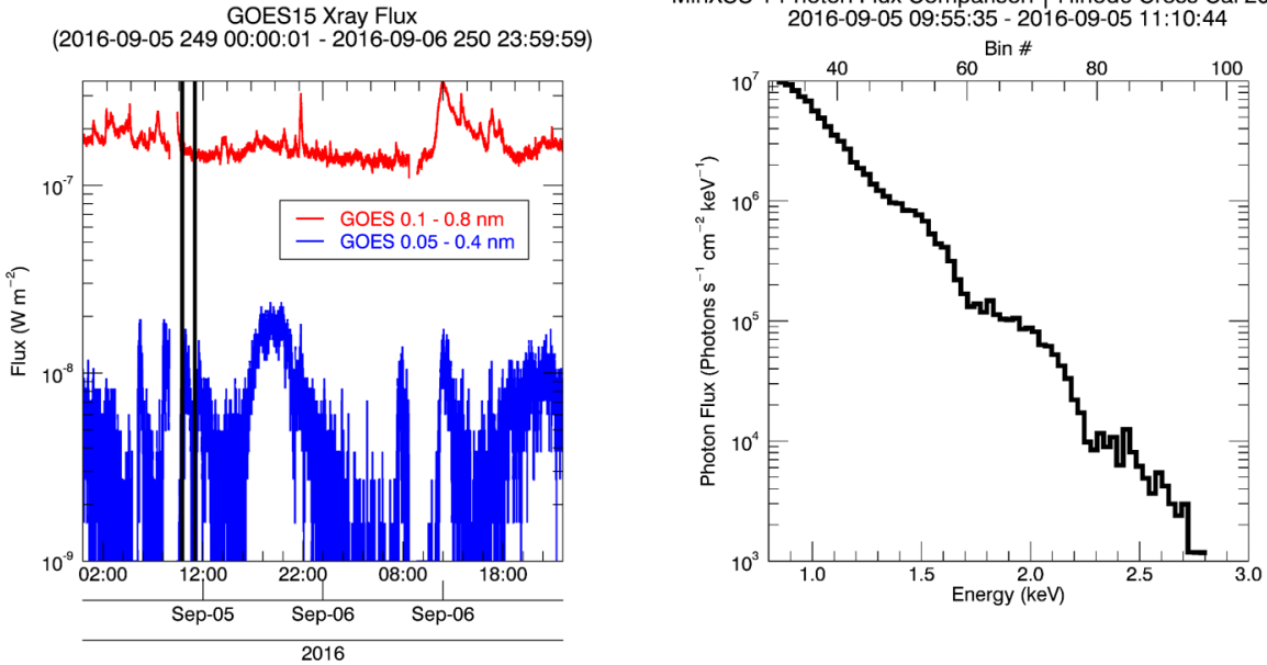
Figure 9.26: MinXSS-1 \leftrightarrow XRT cross-calibration on 2016 September 5. Left plot: GOES 0.1 - 0.8 nm (red) and 0.05 - 0.4 nm (blue) energy fluxes vs. time. The black vertical lines indicate the time range that MinXSS-1 observations were averaged over. The Sun was fairly ‘quiet’. Right plot: X123 directly derived (‘inverted’) photon flux incident on the X123 aperture.
