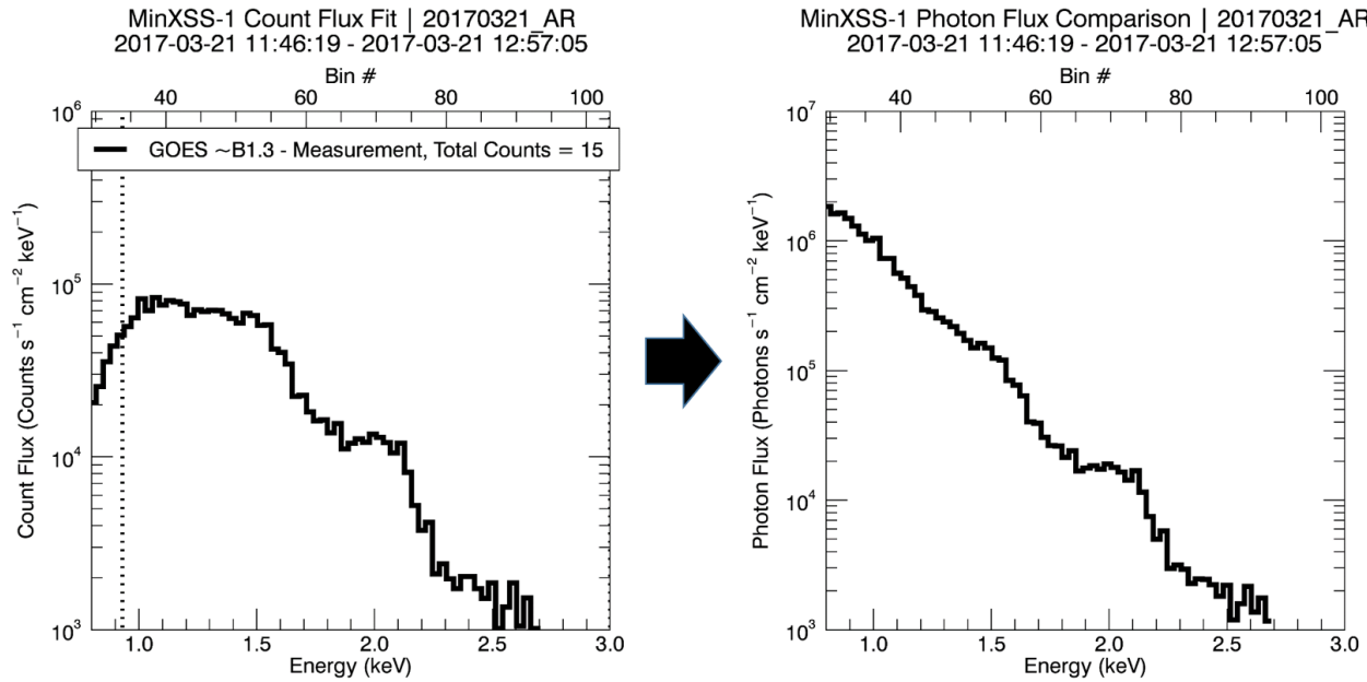
Figure 10.2: Left plot: The estimated active region contribution to the MinXSS-1 X123 count flux and is the difference between the count rate in the 2017 March 21 spectra and the averaged 2017 March 14 - 16 spectra. Right plot: Active region photon flux incident on the X123 aperture, derived from the count flux measurements.
