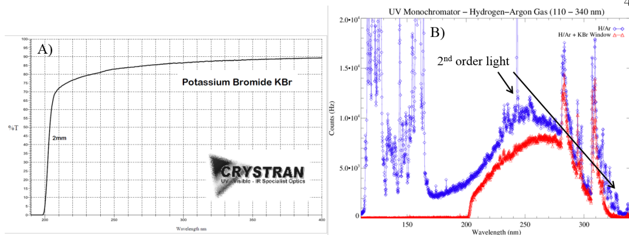
Figure 1. A) Transmission curve for a KBr window. B) Background subtracted intensity from our Hydrogen-Argon (H/Ar - 35%/65% mix) discharge gas with second order diffracted light for \lambda > 220 nm, in blue diamonds. Overplotted is the resultant intensity of the H/Ar with the KBr window, the red triangles. The second order light for \lambda > 220 nm has been attenuated and light for \lambda < 200 nm has been completely removed.
