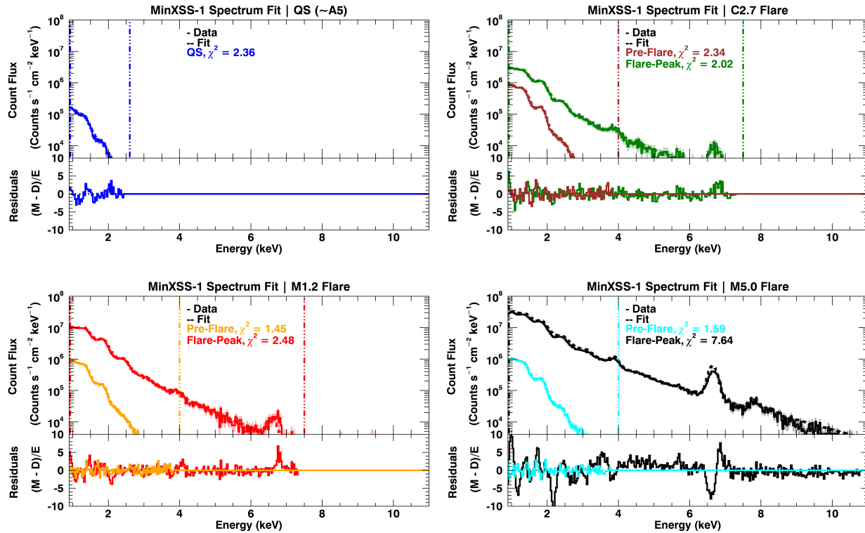
Figure 9.9: MinXSS-1 X123 count flux solar measurements (solid lines) with the best fit spectra overlaid (dashed lines), for temperature and emission measures derived using the OSPEX suite. The residuals are listed also ( M = \text{model} , D = \text{data} , and E = \text{uncertainty} ). The shaded regions indicate the uncertainties in the count flux. A 2T model with select elemental abundance fit separately (2TAllFree). The best fit parameters with their uncertainties are listed in Table 9.3 and Table 9.4. There is a 2T model used for non-large-flaring times (QS and pre-flare) and an additional 2T model is added to compensate for the radiative enhancement during the flare-peak times. The vertical dash-dot-dot-dot lines show the high and low energy limits for the spectral fits.
