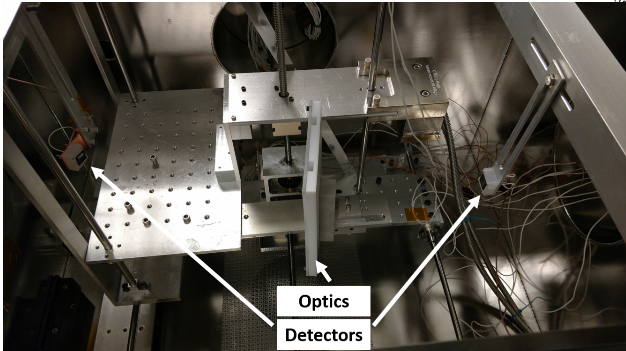
Figure 5.9: Inside the LASP CTE3 chamber. The Si-photodiodes are Opto Diode AXUV100G and flight spares.
