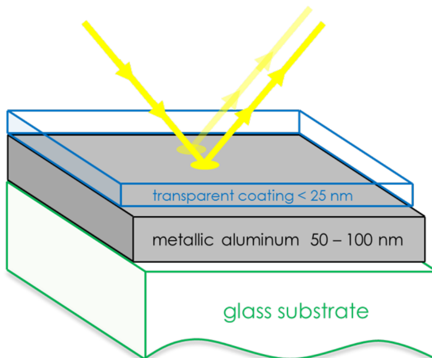
Figure 3.2: Diagram depicting the general mirror architecture implemented in this dissertation. The substrate is either glass or silicon. The transparent coatings discussed include magnesium fluoride ( \text{MgF}_2 ), lithium fluoride ( \text{LiF} ) and the main focus of this dissertation, aluminum fluoride ( \text{AlF}_3 ).
