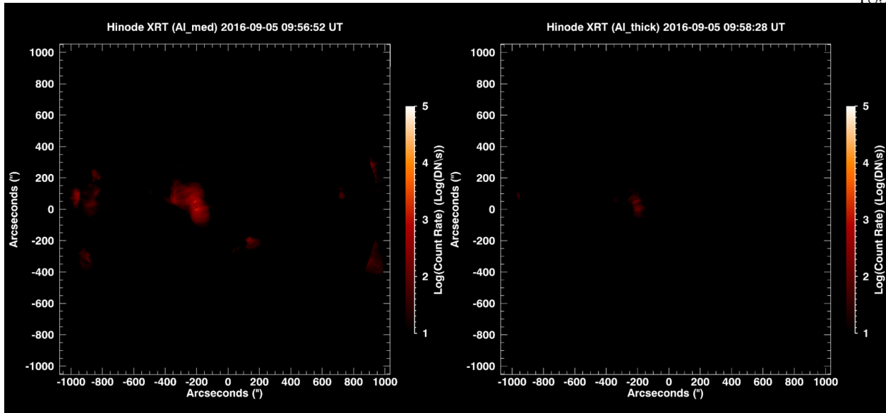
Figure 9.24: MinXSS-1 \leftrightarrow XRT cross-calibration on 2016 September 5. Log-scaled count rate XRT Al-med and Al-thick full Sun images. These ‘thicker’ aluminum filters are mostly sensitive to photons between 0.6 - 1.6 keV and generally probes plasma for T \geq 2 MK. Active region emission is readily observed in these filter images.
