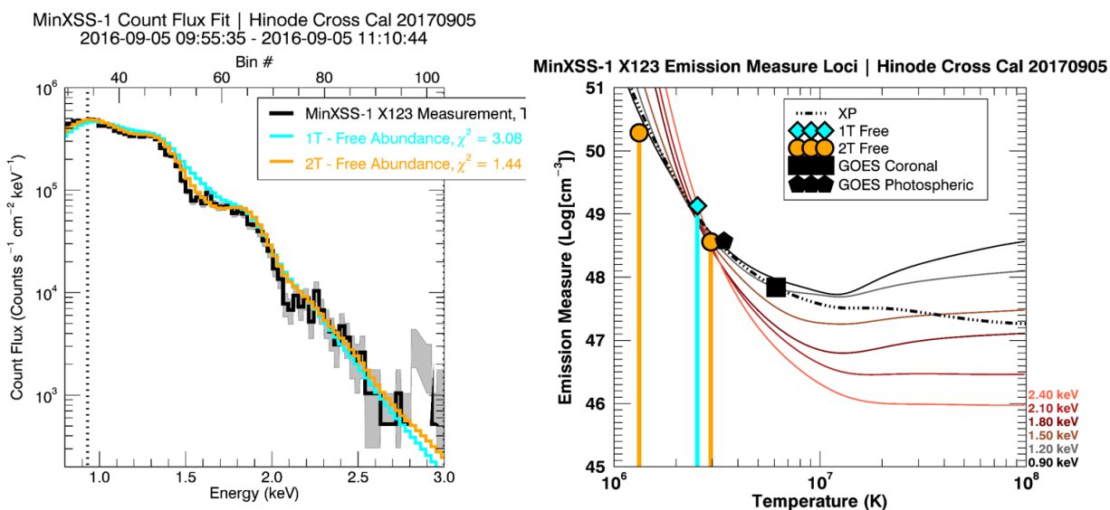
Figure 9.27: MinXSS-1 \leftrightarrow XRT cross-calibration on 2016 September 5. Left plot: MinXSS-1 X123 count flux and OSPEX 1T and 2T spectral fits. Right plot: X123 and XP em loci with the 1T, 2T Free OSPEX fits and the GOES photospheric (pentagon) and coronal (square) values overplotted.
