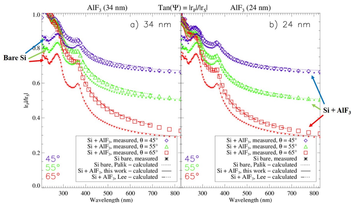
Figure 5.6: Measurements of \tan \Psi , the ratio of the modulus of the p to s polarization state Fresnel coefficients for 34 nm (Panel a) and 24 nm (Panel b) of \text{AlF}_3 on Si wafers at \theta = 45^\circ, 55^\circ and 65^\circ (blue, green and red symbols respectively). Values near unity indicate even amounts of reflected light for both polarization states. Deviations from unity mean different amounts of each state are reflected. For reference, bare Si substrate (with probable native oxide) measurements are over-plotted with small symbols (asterisks) and calculations from the Palik archive optical constants (dotted line). Measurements agree in general with optical constant calculations from ‘this work’ (solid line, ALD) and well with Lee (dash-dotted line, magnetron - sputtered). \Delta combined with \Psi describe polarization state changes (between linear, circular and/or elliptical) upon reflection from our Si + \text{AlF}_3 combination.
