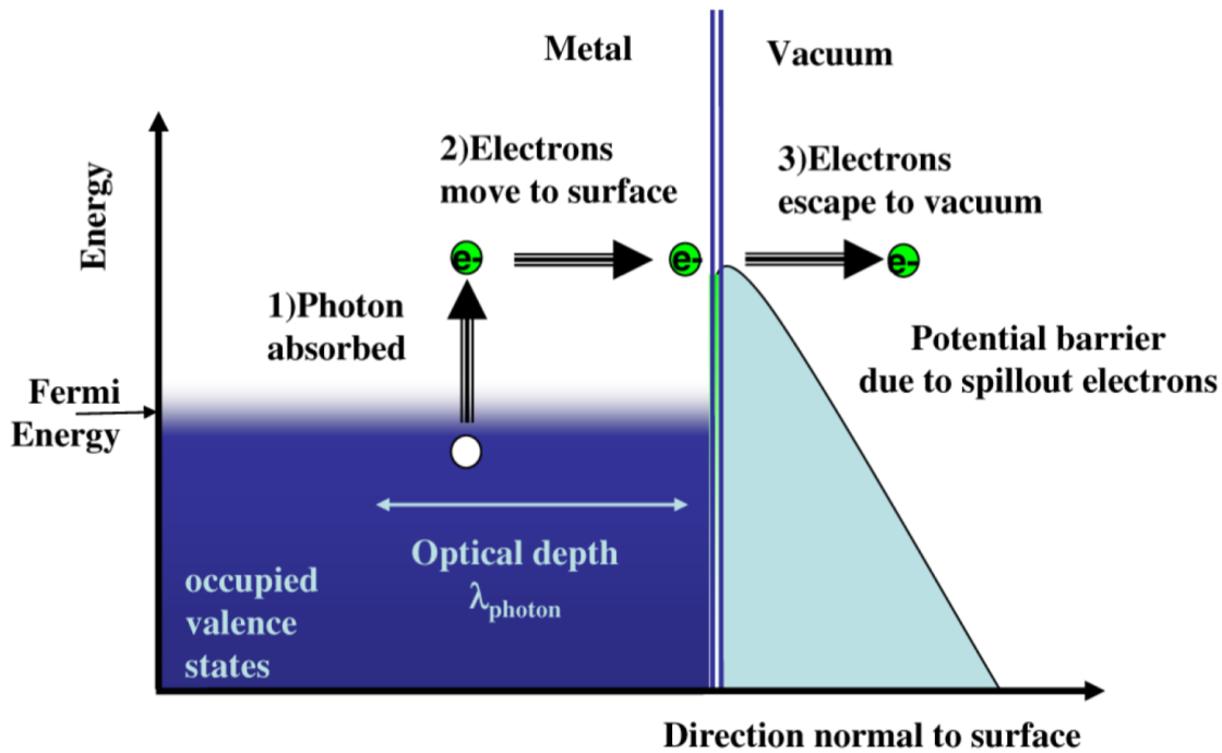
Figure 8.10: Diagram displaying the basic processes assumed in the Spicer model used to estimate the X123 Be window photoelectron contribution. Figure adapted from Dowell and Schmege 2009 [41].
