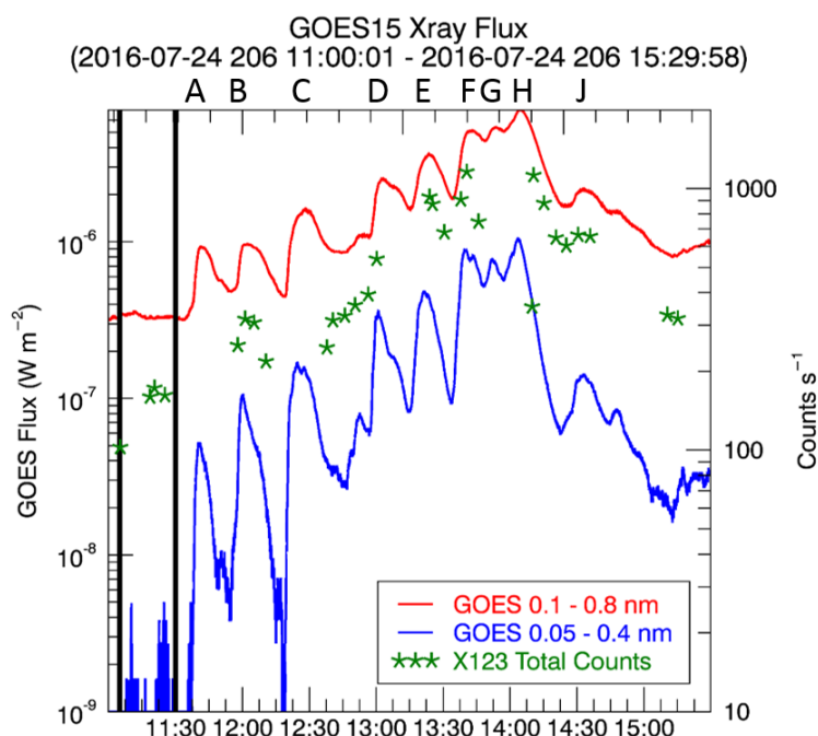
Figure 11.1: GOES XRS 0.1 - 0.8 nm (red line) and 0.05 - 0.4 (blue line) nm flux time series with the X123 total counts overplotted (green asterisks). The 5 minute averages X123 total counts follows the general trend of the GOES XRS measurements.
